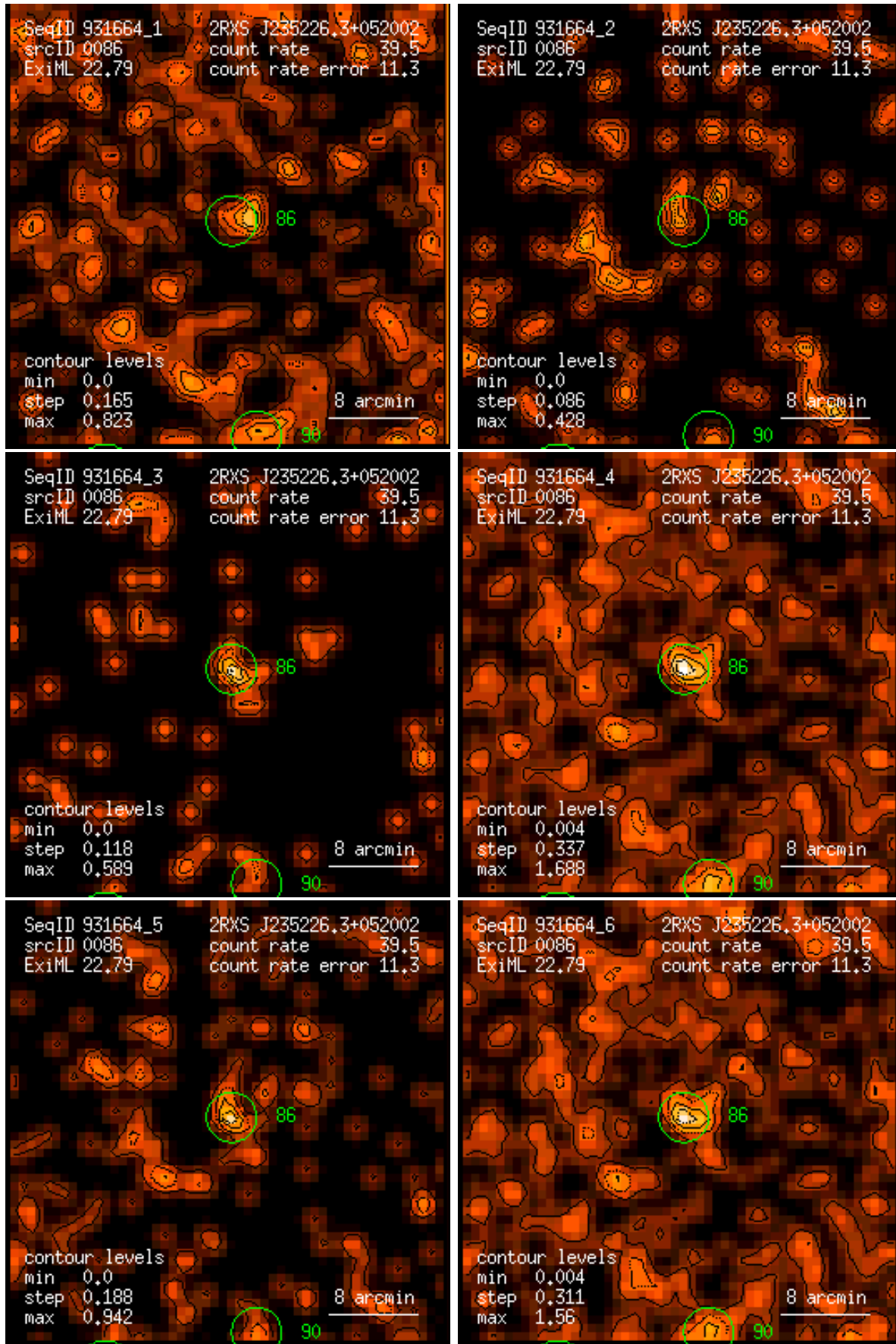
Figure 86: RASS 931664: detection 0086: band rate images, Gaussian filter: (1) PSPC channels 11 – 41, (2) 52 – 90, (3) 91 – 201, (4) 11 – 235, (5) 52 – 201, (6) 11 – 201. Broad band rates in counts/ks. Band rate contour levels in counts/ks/arcmin 2 .
