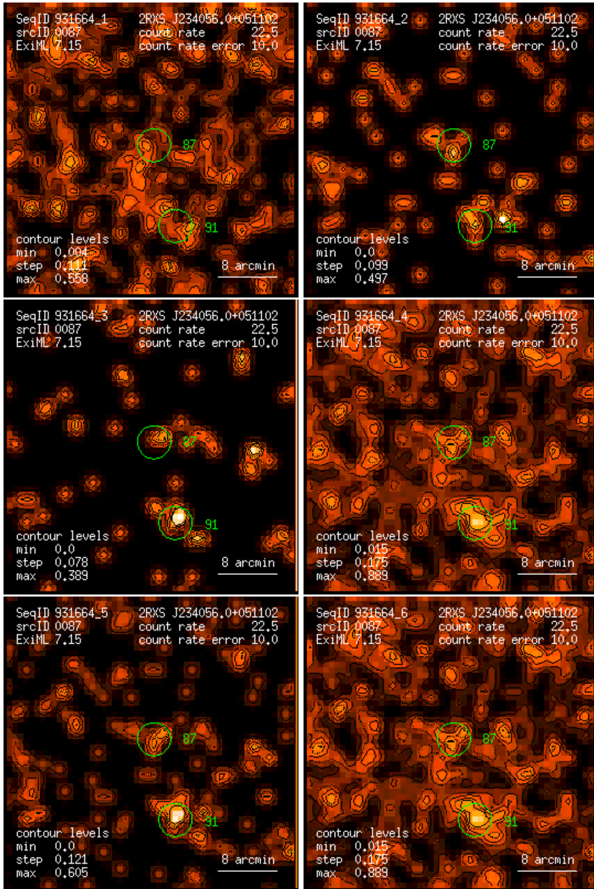
Figure 87: RASS 931664: detection 0087: band rate images, Gaussian filter: (1) PSPC channels 11 – 41, (2) 52 – 90, (3) 91 – 201, (4) 11 – 235, (5) 52 – 201, (6) 11 – 201. Broad band rates in counts/ks. Band rate contour levels in counts/ks/arcmin 2 .
