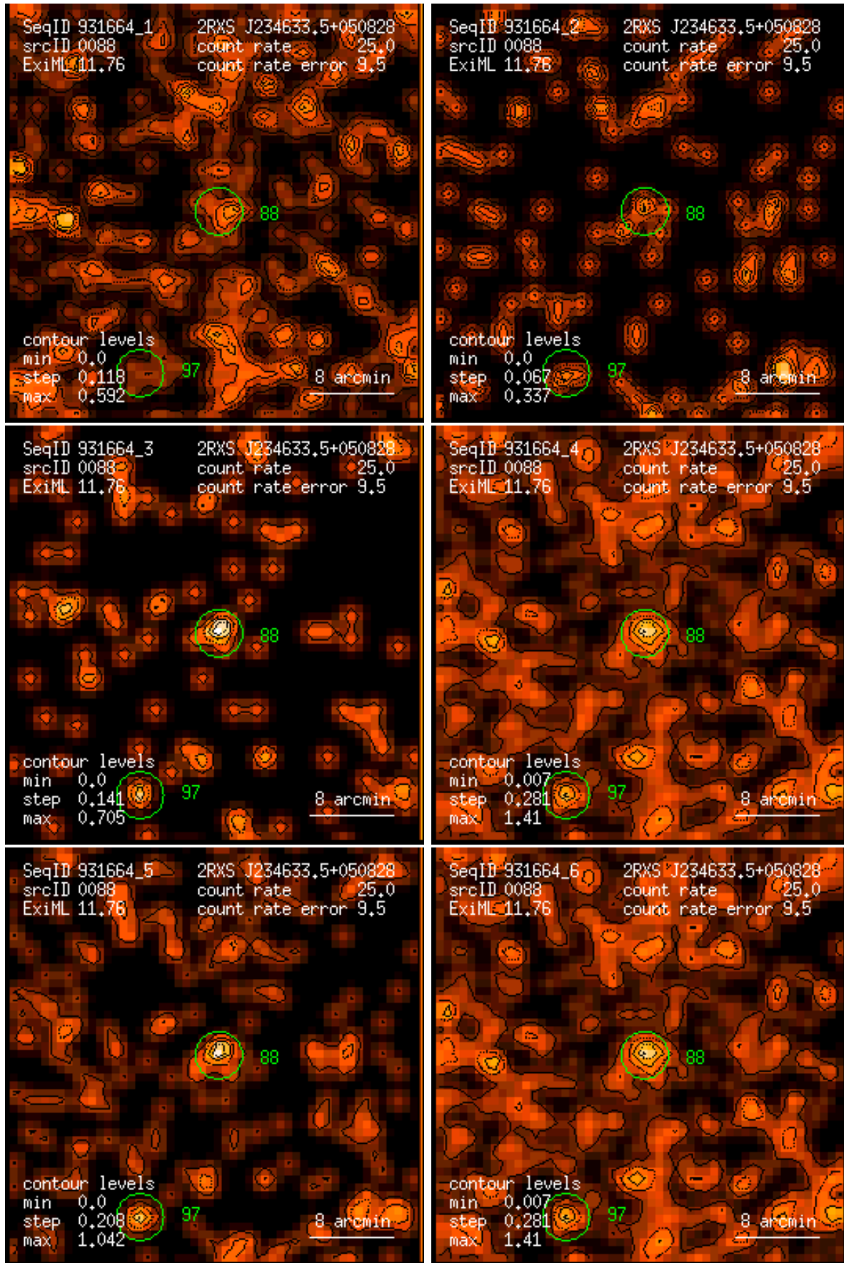
Figure 88: RASS 931664: detection 0088: band rate images, Gaussian filter: (1) PSPC channels 11 – 41, (2) 52 – 90, (3) 91 – 201, (4) 11 – 235, (5) 52 – 201, (6) 11 – 201. Broad band rates in counts/ks. Band rate contour levels in counts/ks/arcmin 2 .
