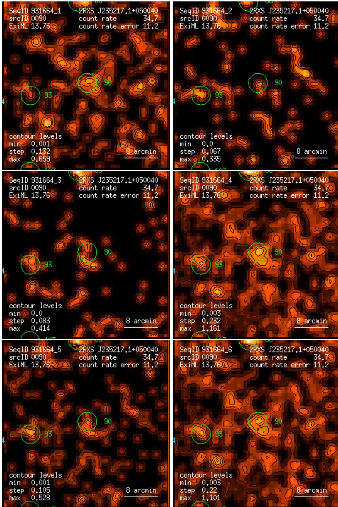
Figure 90: RASS 931664: detection 0090: band rate images, Gaussian filter: (1) PSPC channels 11 – 41, (2) 52 – 90, (3) 91 – 201, (4) 11 – 235, (5) 52 – 201, (6) 11 – 201. Broad band rates in counts/ks. Band rate contour levels in counts/ks/arcmin 2 .
