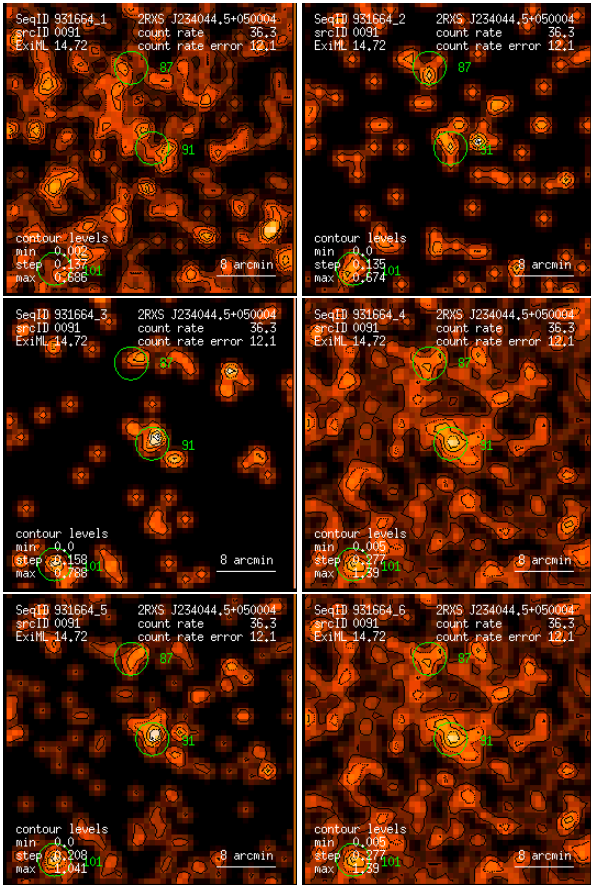
Figure 91: RASS 931664: detection 0091: band rate images, Gaussian filter: (1) PSPC channels 11 – 41, (2) 52 – 90, (3) 91 – 201, (4) 11 – 235, (5) 52 – 201, (6) 11 – 201. Broad band rates in counts/ks. Band rate contour levels in counts/ks/arcmin 2 .
