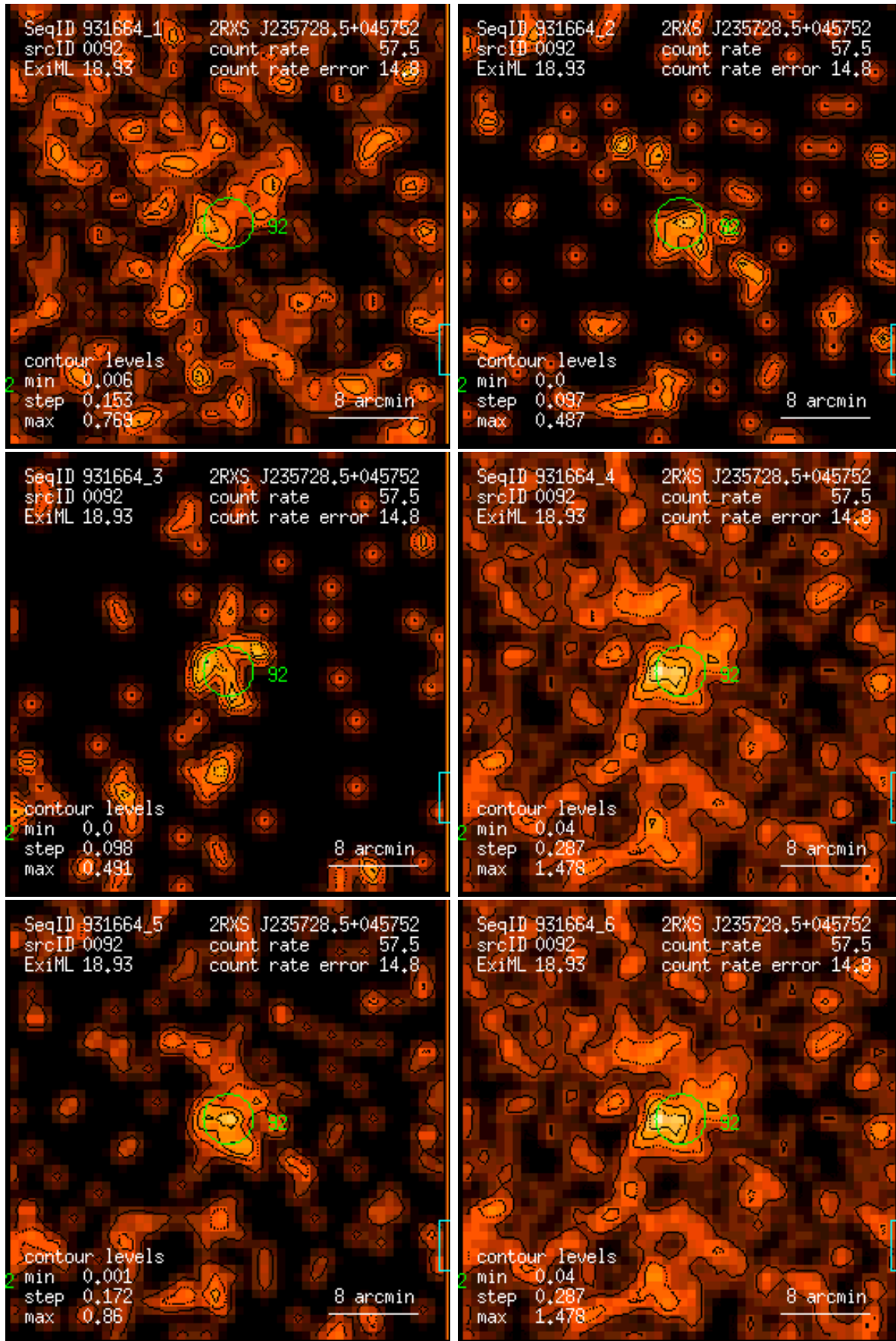
Figure 92: RASS 931664: detection 0092: band rate images, Gaussian filter: (1) PSPC channels 11 – 41, (2) 52 – 90, (3) 91 – 201, (4) 11 – 235, (5) 52 – 201, (6) 11 – 201. Broad band rates in counts/ks. Band rate contour levels in counts/ks/arcmin 2 .
