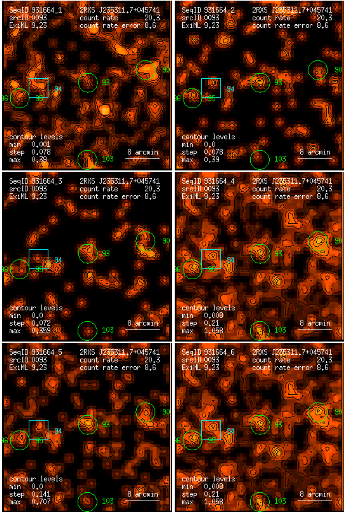
Figure 93: RASS 931664: detection 0093: band rate images, Gaussian filter: (1) PSPC channels 11 – 41, (2) 52 – 90, (3) 91 – 201, (4) 11 – 235, (5) 52 – 201, (6) 11 – 201. Broad band rates in counts/ks. Band rate contour levels in counts/ks/arcmin 2 .
