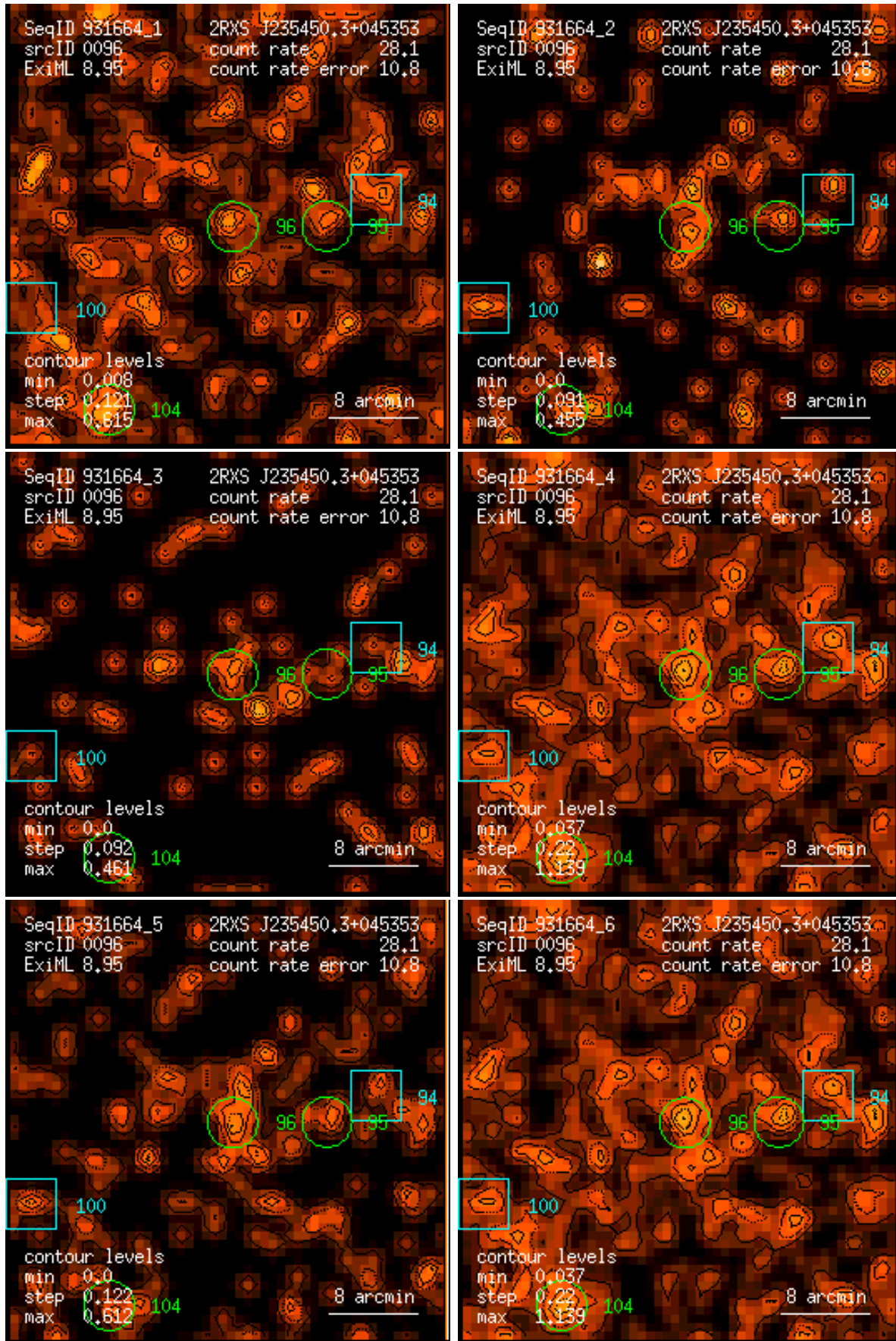
Figure 96: RASS 931664: detection 0096: band rate images, Gaussian filter: (1) PSPC channels 11 – 41, (2) 52 – 90, (3) 91 – 201, (4) 11 – 235, (5) 52 – 201, (6) 11 – 201. Broad band rates in counts/ks. Band rate contour levels in counts/ks/arcmin 2 .
