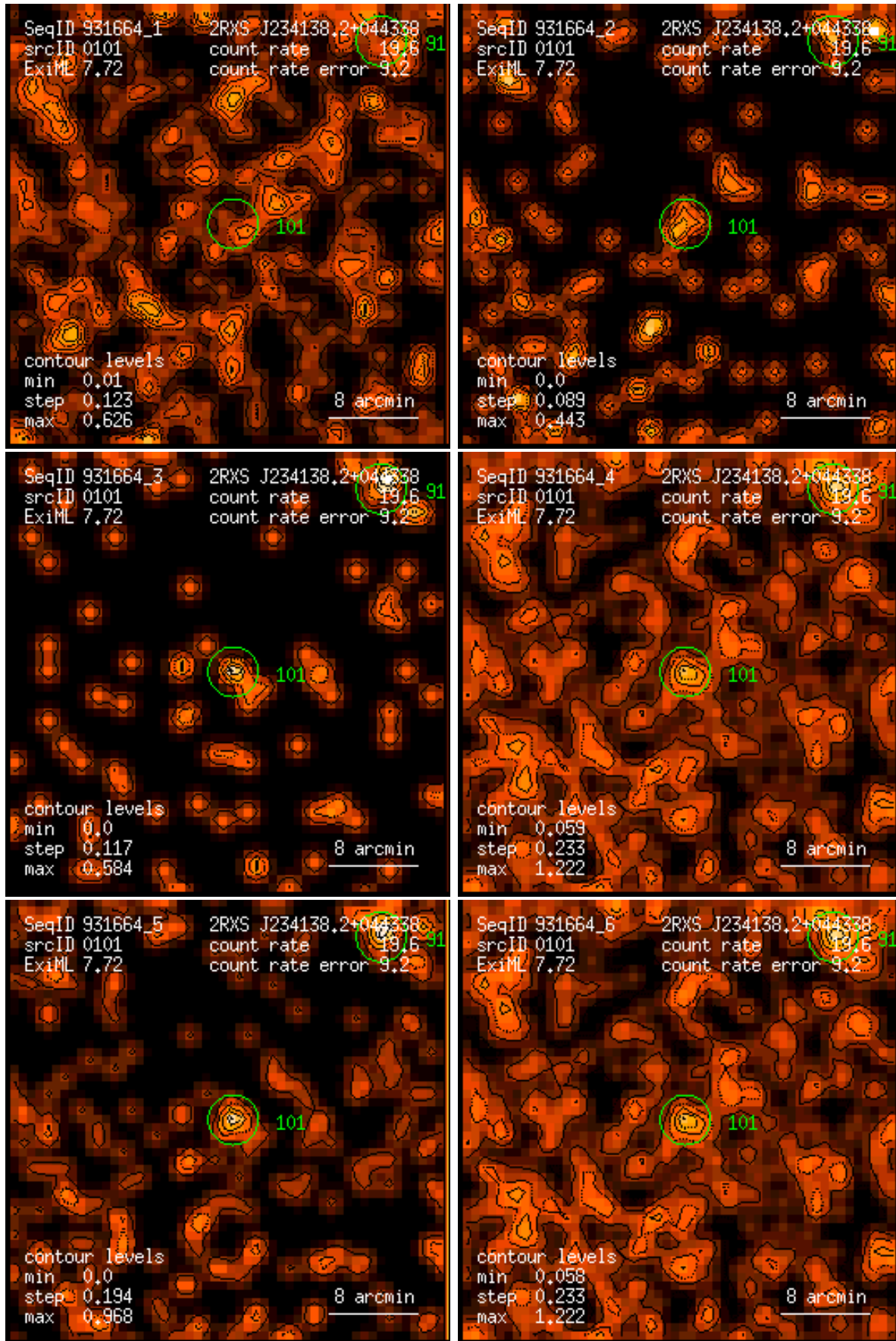
Figure 101: RASS 931664: detection 0101: band rate images, Gaussian filter: (1) PSPC channels 11 – 41, (2) 52 – 90, (3) 91 – 201, (4) 11 – 235, (5) 52 – 201, (6) 11 – 201. Broad band rates in counts/ks. Band rate contour levels in counts/ks/arcmin 2 .
