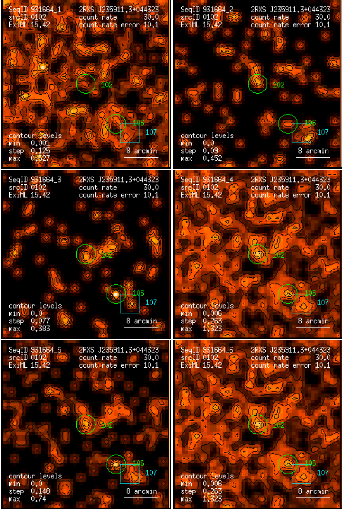
Figure 102: RASS 931664: detection 0102: band rate images, Gaussian filter: (1) PSPC channels 11 – 41, (2) 52 – 90, (3) 91 – 201, (4) 11 – 235, (5) 52 – 201, (6) 11 – 201. Broad band rates in counts/ks. Band rate contour levels in counts/ks/arcmin 2 .
