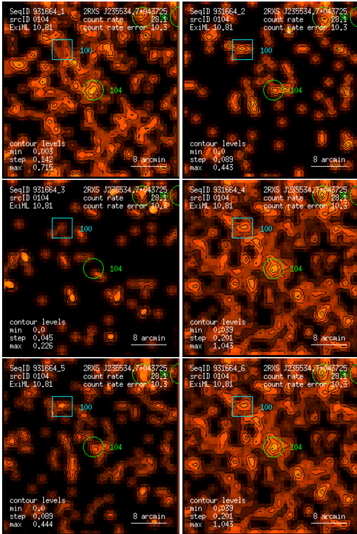
Figure 104: RASS 931664: detection 0104: band rate images, Gaussian filter: (1) PSPC channels 11 – 41, (2) 52 – 90, (3) 91 – 201, (4) 11 – 235, (5) 52 – 201, (6) 11 – 201. Broad band rates in counts/ks. Band rate contour levels in counts/ks/arcmin 2 .
