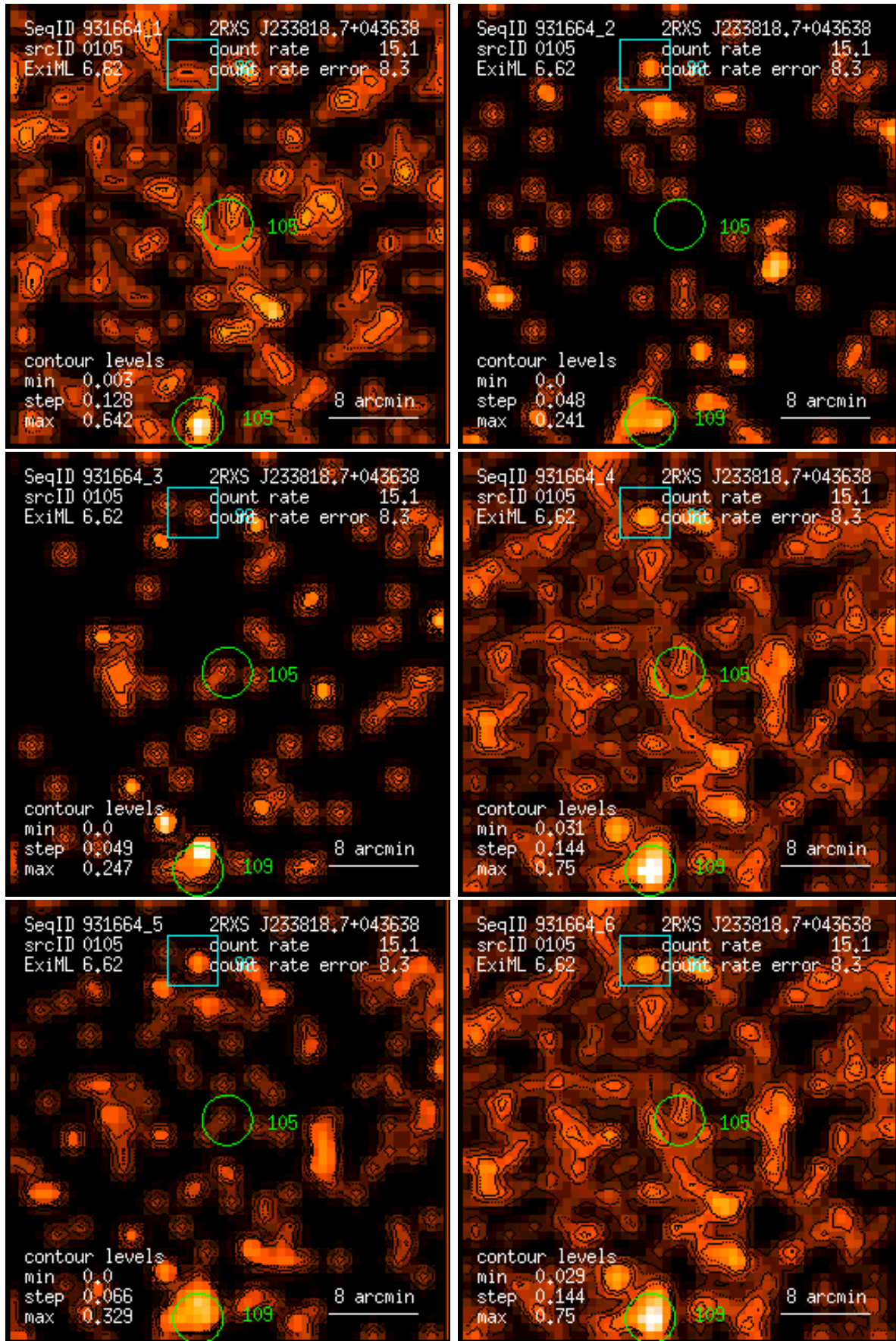
Figure 105: RASS 931664: detection 0105: band rate images, Gaussian filter: (1) PSPC channels 11 – 41, (2) 52 – 90, (3) 91 – 201, (4) 11 – 235, (5) 52 – 201, (6) 11 – 201. Broad band rates in counts/ks. Band rate contour levels in counts/ks/arcmin 2 .
