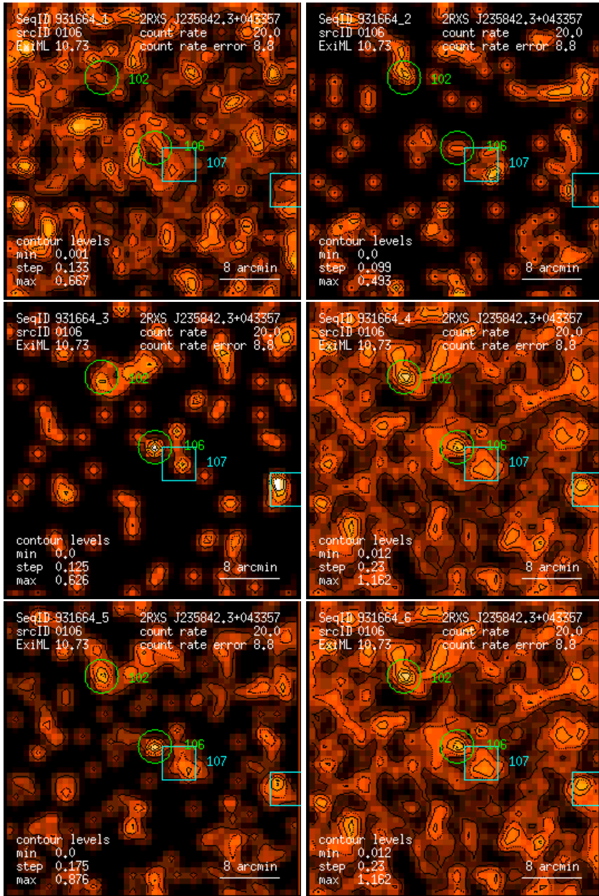
Figure 106: RASS 931664: detection 0106: band rate images, Gaussian filter: (1) PSPC channels 11 – 41, (2) 52 – 90, (3) 91 – 201, (4) 11 – 235, (5) 52 – 201, (6) 11 – 201. Broad band rates in counts/ks. Band rate contour levels in counts/ks/arcmin 2 .
