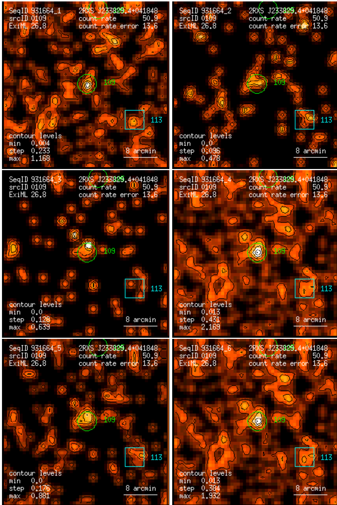
Figure 109: RASS 931664: detection 0109: band rate images, Gaussian filter: (1) PSPC channels 11 – 41, (2) 52 – 90, (3) 91 – 201, (4) 11 – 235, (5) 52 – 201, (6) 11 – 201. Broad band rates in counts/ks. Band rate contour levels in counts/ks/arcmin 2 .
