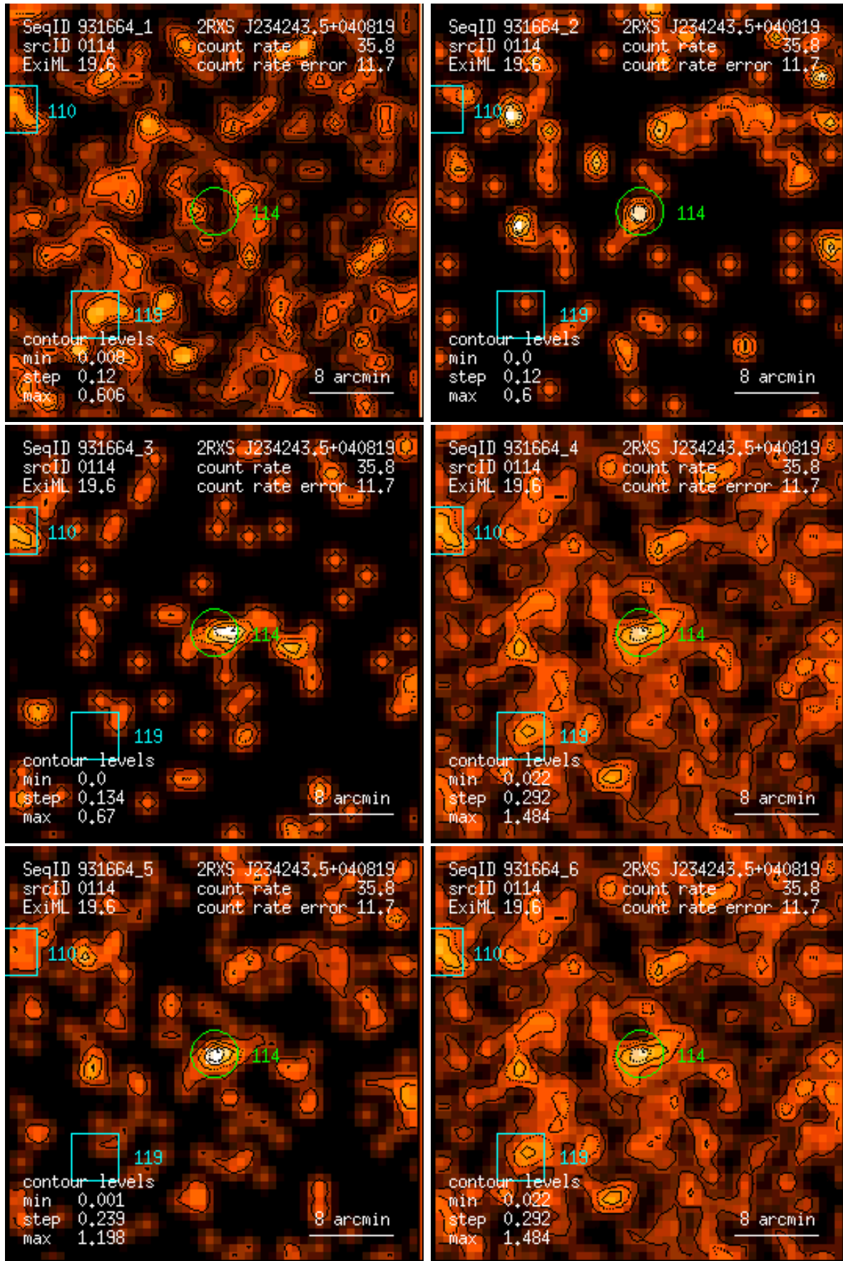
Figure 114: RASS 931664: detection 0114: band rate images, Gaussian filter: (1) PSPC channels 11 – 41, (2) 52 – 90, (3) 91 – 201, (4) 11 – 235, (5) 52 – 201, (6) 11 – 201. Broad band rates in counts/ks. Band rate contour levels in counts/ks/arcmin 2 .
