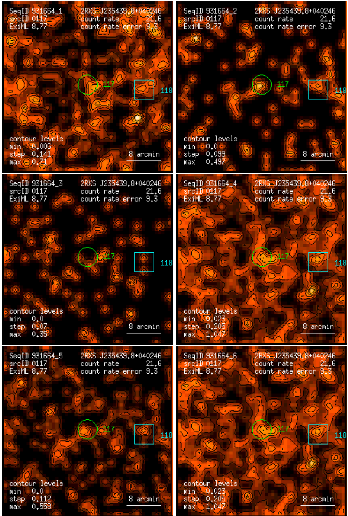
Figure 117: RASS 931664: detection 0117: band rate images, Gaussian filter: (1) PSPC channels 11 – 41, (2) 52 – 90, (3) 91 – 201, (4) 11 – 235, (5) 52 – 201, (6) 11 – 201. Broad band rates in counts/ks. Band rate contour levels in counts/ks/arcmin 2 .
