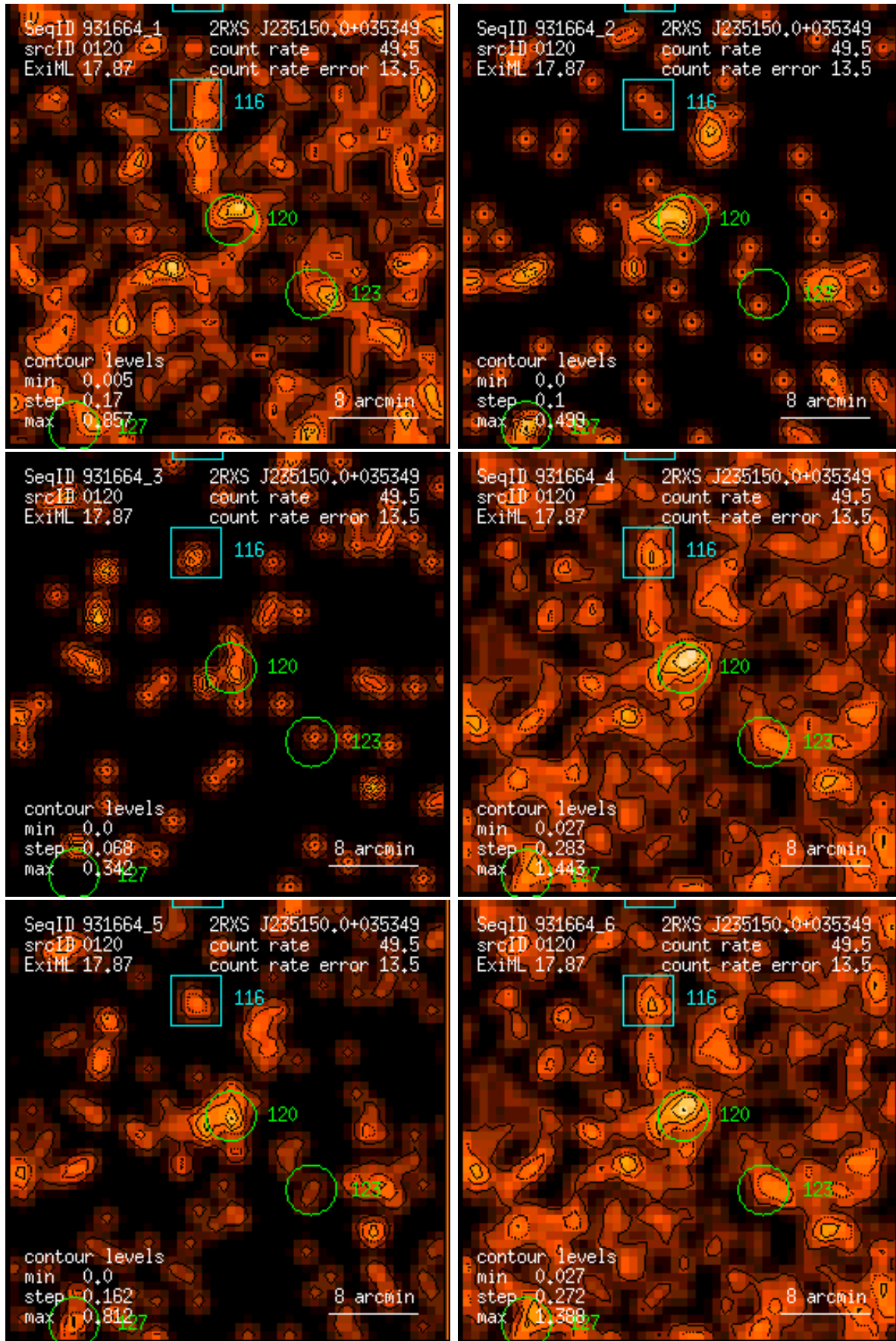
Figure 120: RASS 931664: detection 0120: band rate images, Gaussian filter: (1) PSPC channels 11 – 41, (2) 52 – 90, (3) 91 – 201, (4) 11 – 235, (5) 52 – 201, (6) 11 – 201. Broad band rates in counts/ks. Band rate contour levels in counts/ks/arcmin 2 .
