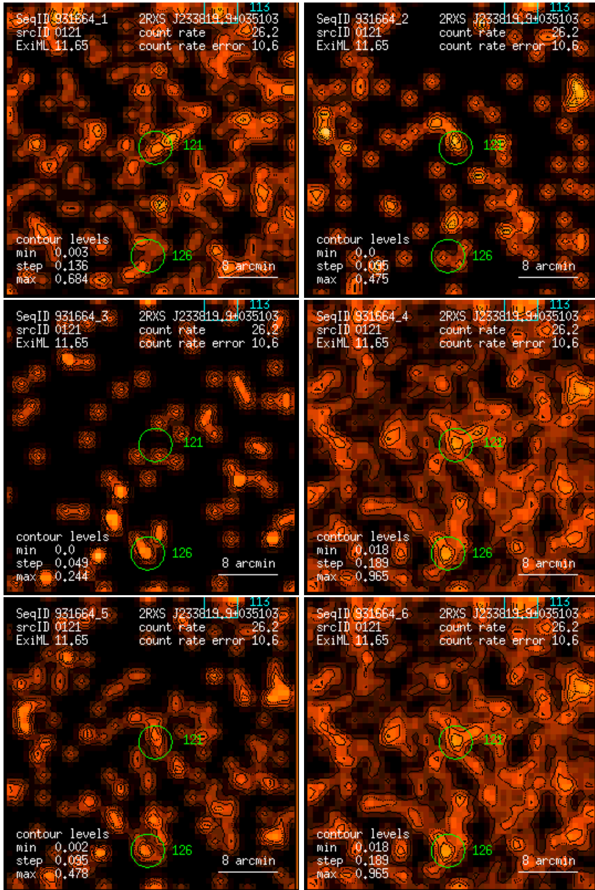
Figure 121: RASS 931664: detection 0121: band rate images, Gaussian filter: (1) PSPC channels 11 – 41, (2) 52 – 90, (3) 91 – 201, (4) 11 – 235, (5) 52 – 201, (6) 11 – 201. Broad band rates in counts/ks. Band rate contour levels in counts/ks/arcmin 2 .
