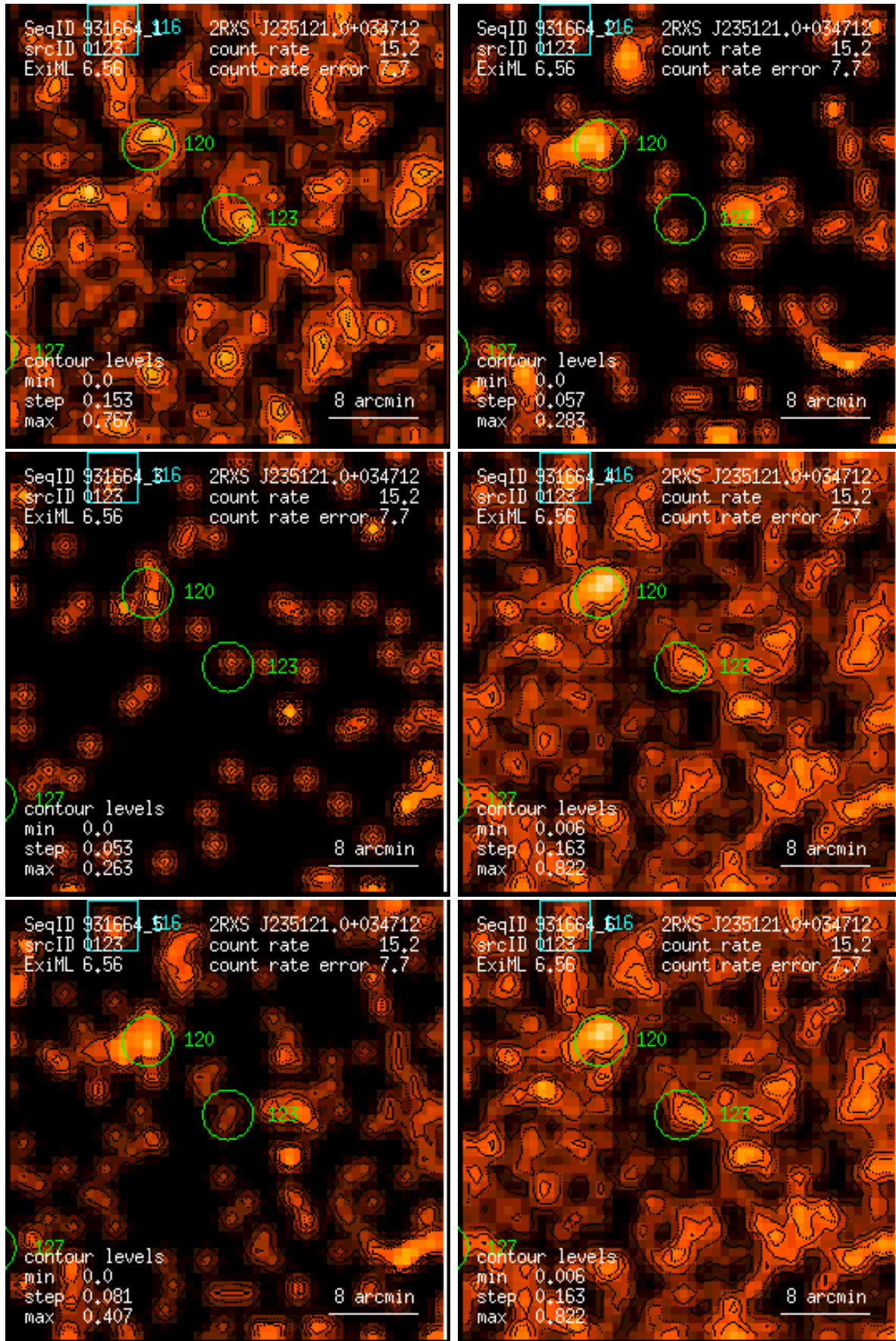
Figure 123: RASS 931664: detection 0123: band rate images, Gaussian filter: (1) PSPC channels 11 – 41, (2) 52 – 90, (3) 91 – 201, (4) 11 – 235, (5) 52 – 201, (6) 11 – 201. Broad band rates in counts/ks. Band rate contour levels in counts/ks/arcmin 2 .
