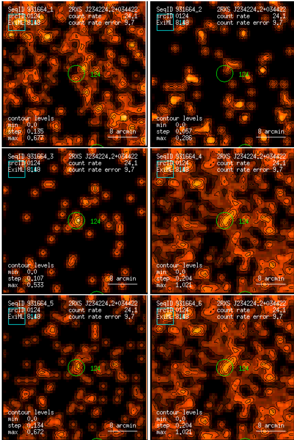
Figure 124: RASS 931664: detection 0124: band rate images, Gaussian filter: (1) PSPC channels 11 – 41, (2) 52 – 90, (3) 91 – 201, (4) 11 – 235, (5) 52 – 201, (6) 11 – 201. Broad band rates in counts/ks. Band rate contour levels in counts/ks/arcmin 2 .
