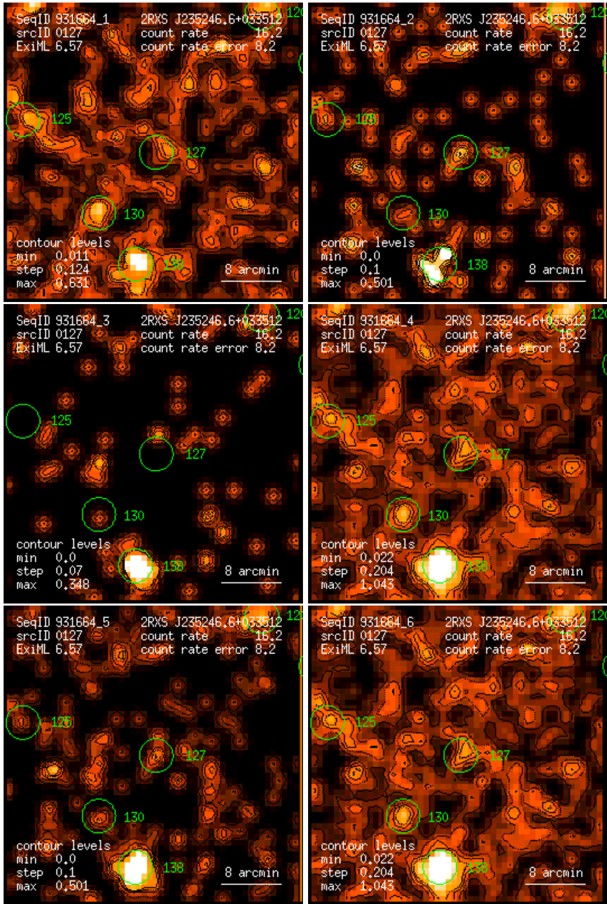
Figure 127: RASS 931664: detection 0127: band rate images, Gaussian filter: (1) PSPC channels 11 – 41, (2) 52 – 90, (3) 91 – 201, (4) 11 – 235, (5) 52 – 201, (6) 11 – 201. Broad band rates in counts/ks. Band rate contour levels in counts/ks/arcmin 2 .
