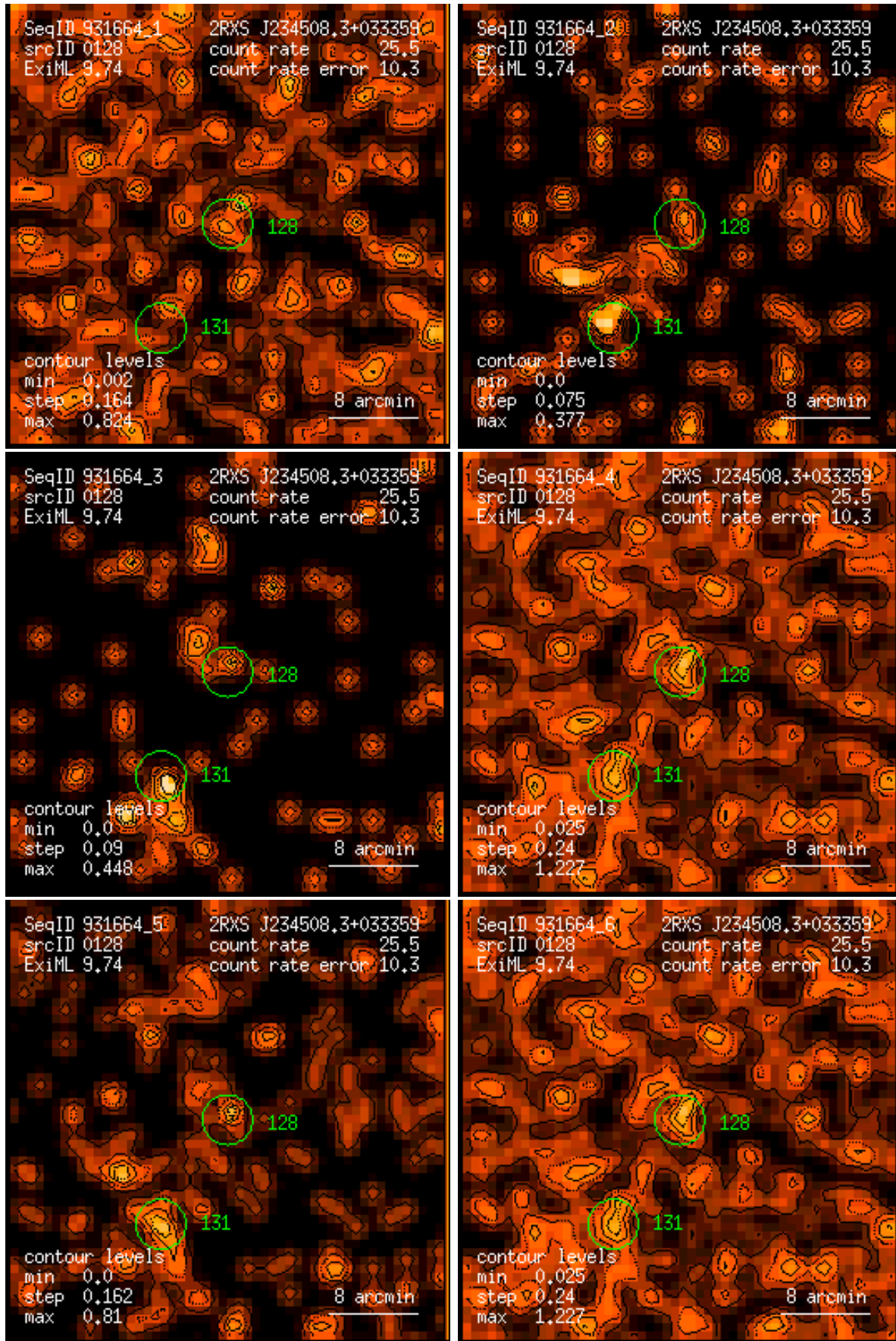
Figure 128: RASS 931664: detection 0128: band rate images, Gaussian filter: (1) PSPC channels 11 – 41, (2) 52 – 90, (3) 91 – 201, (4) 11 – 235, (5) 52 – 201, (6) 11 – 201. Broad band rates in counts/ks. Band rate contour levels in counts/ks/arcmin 2 .
