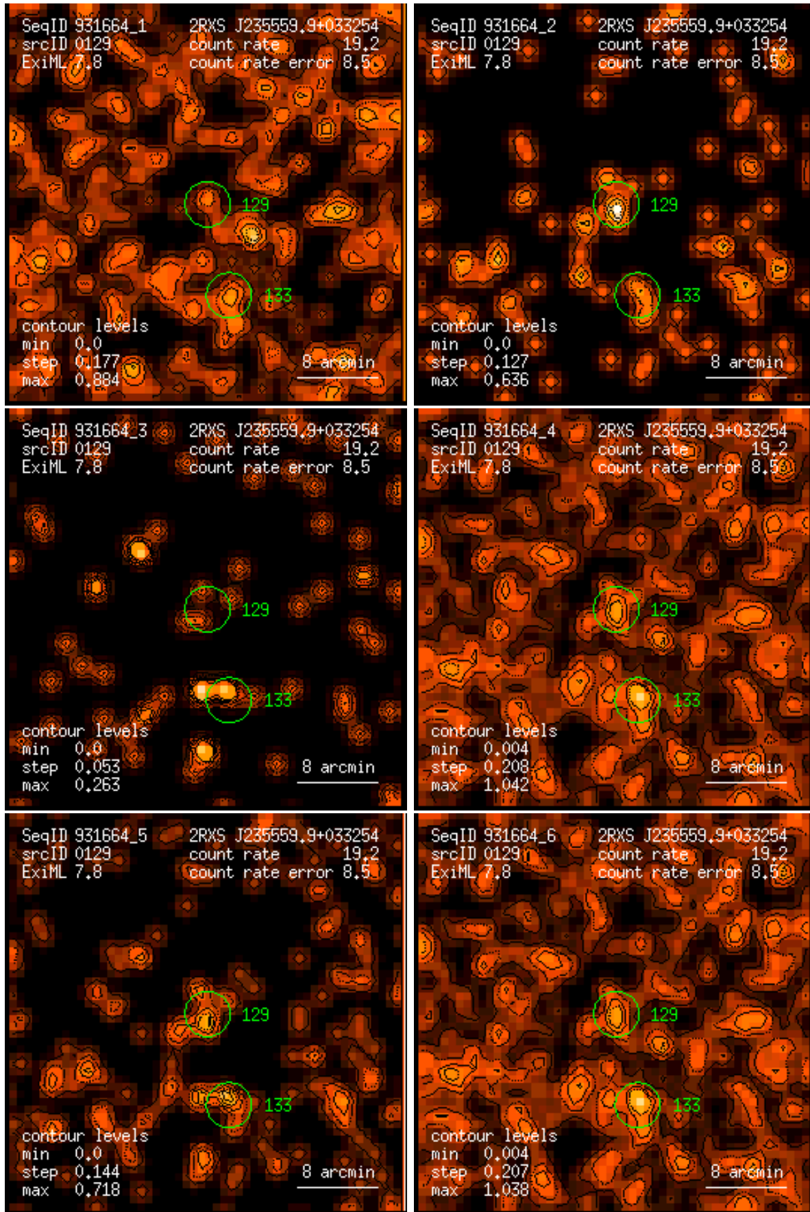
Figure 129: RASS 931664: detection 0129: band rate images, Gaussian filter: (1) PSPC channels 11 – 41, (2) 52 – 90, (3) 91 – 201, (4) 11 – 235, (5) 52 – 201, (6) 11 – 201. Broad band rates in counts/ks. Band rate contour levels in counts/ks/arcmin 2 .
