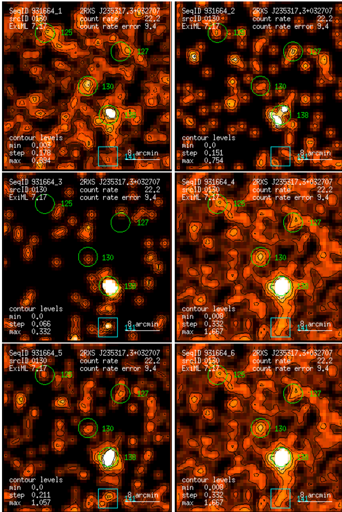
Figure 130: RASS 931664: detection 0130: band rate images, Gaussian filter: (1) PSPC channels 11 – 41, (2) 52 – 90, (3) 91 – 201, (4) 11 – 235, (5) 52 – 201, (6) 11 – 201. Broad band rates in counts/ks. Band rate contour levels in counts/ks/arcmin 2 .
