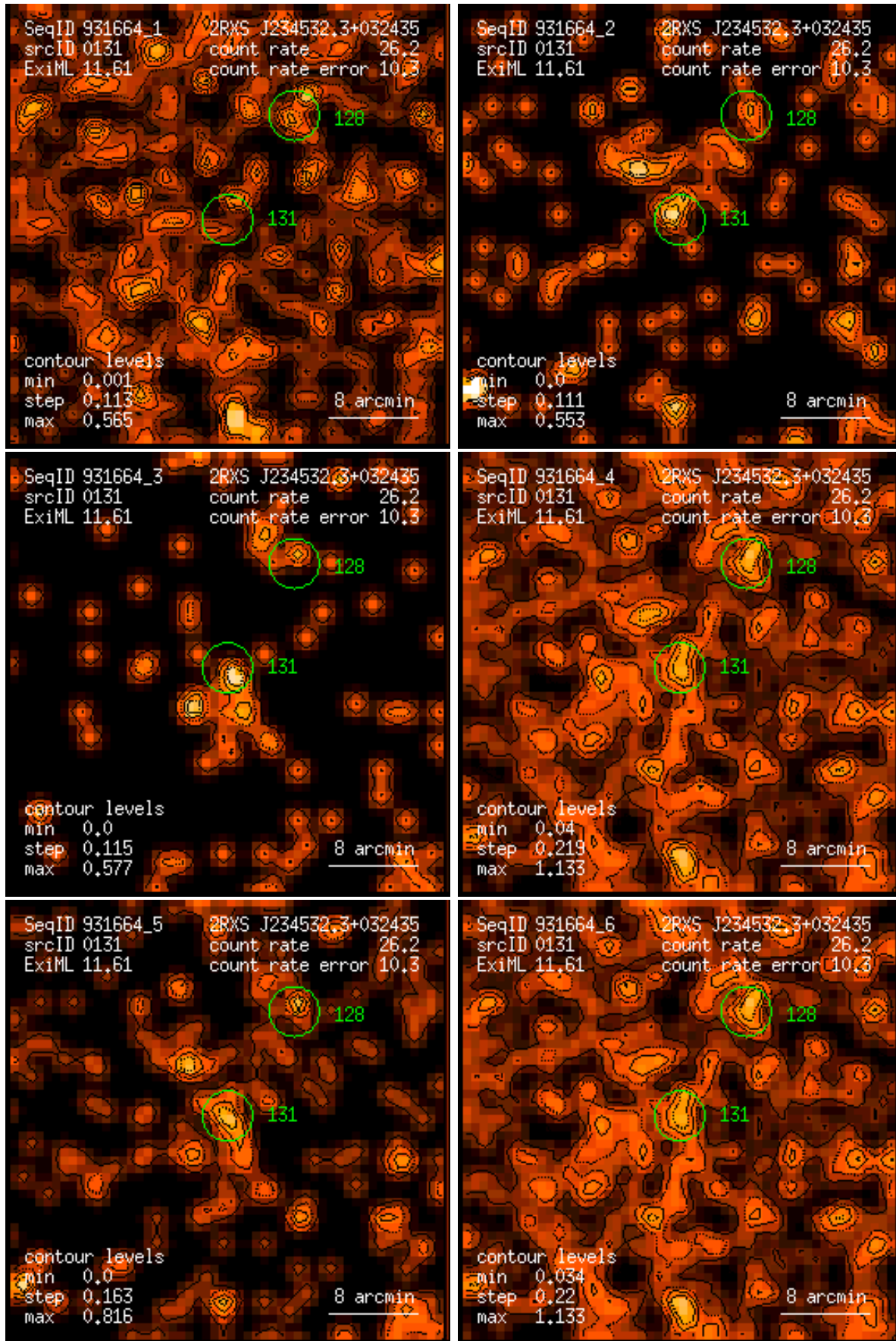
Figure 131: RASS 931664: detection 0131: band rate images, Gaussian filter: (1) PSPC channels 11 – 41, (2) 52 – 90, (3) 91 – 201, (4) 11 – 235, (5) 52 – 201, (6) 11 – 201. Broad band rates in counts/ks. Band rate contour levels in counts/ks/arcmin 2 .
