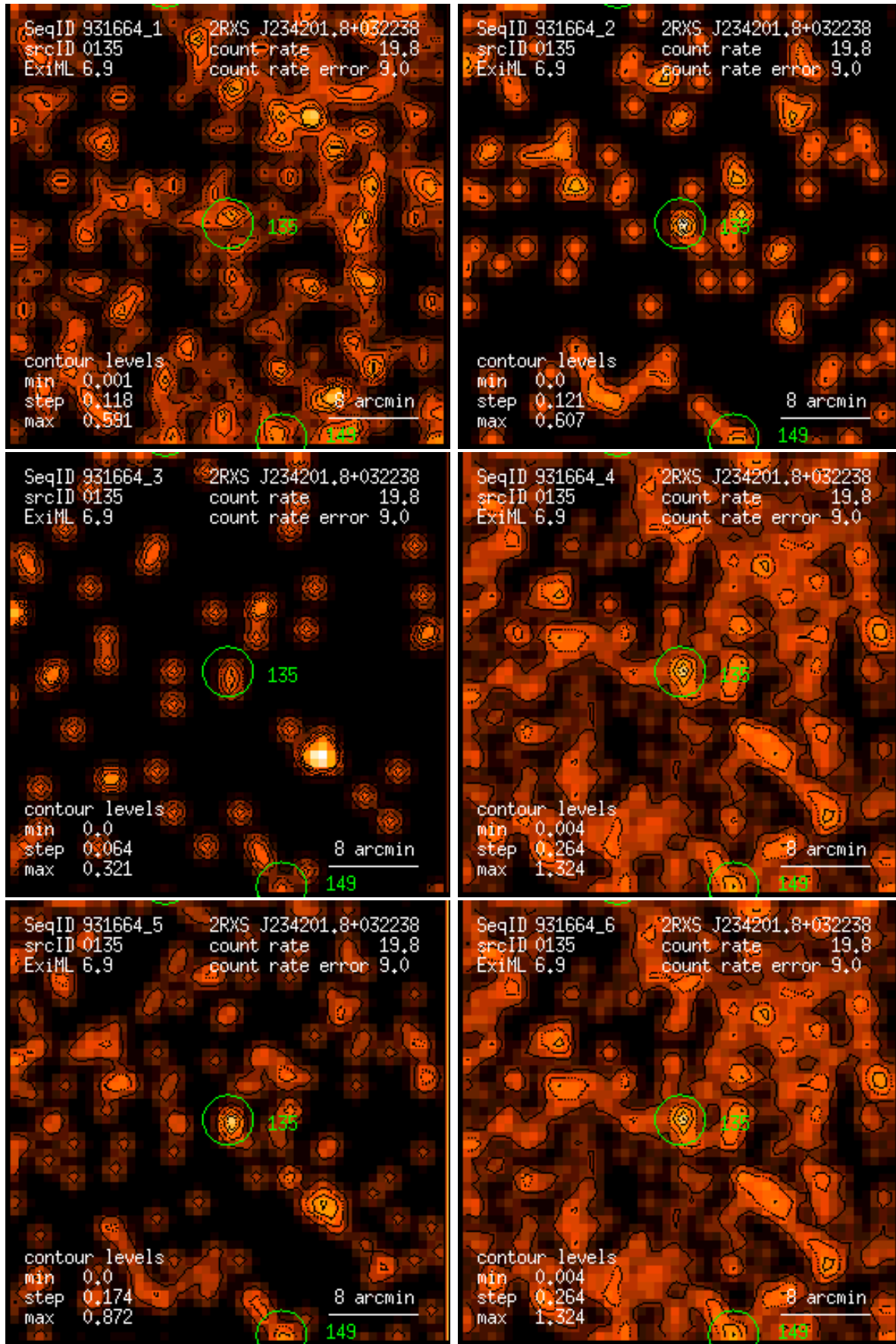
Figure 135: RASS 931664: detection 0135: band rate images, Gaussian filter: (1) PSPC channels 11 – 41, (2) 52 – 90, (3) 91 – 201, (4) 11 – 235, (5) 52 – 201, (6) 11 – 201. Broad band rates in counts/ks. Band rate contour levels in counts/ks/arcmin 2 .
