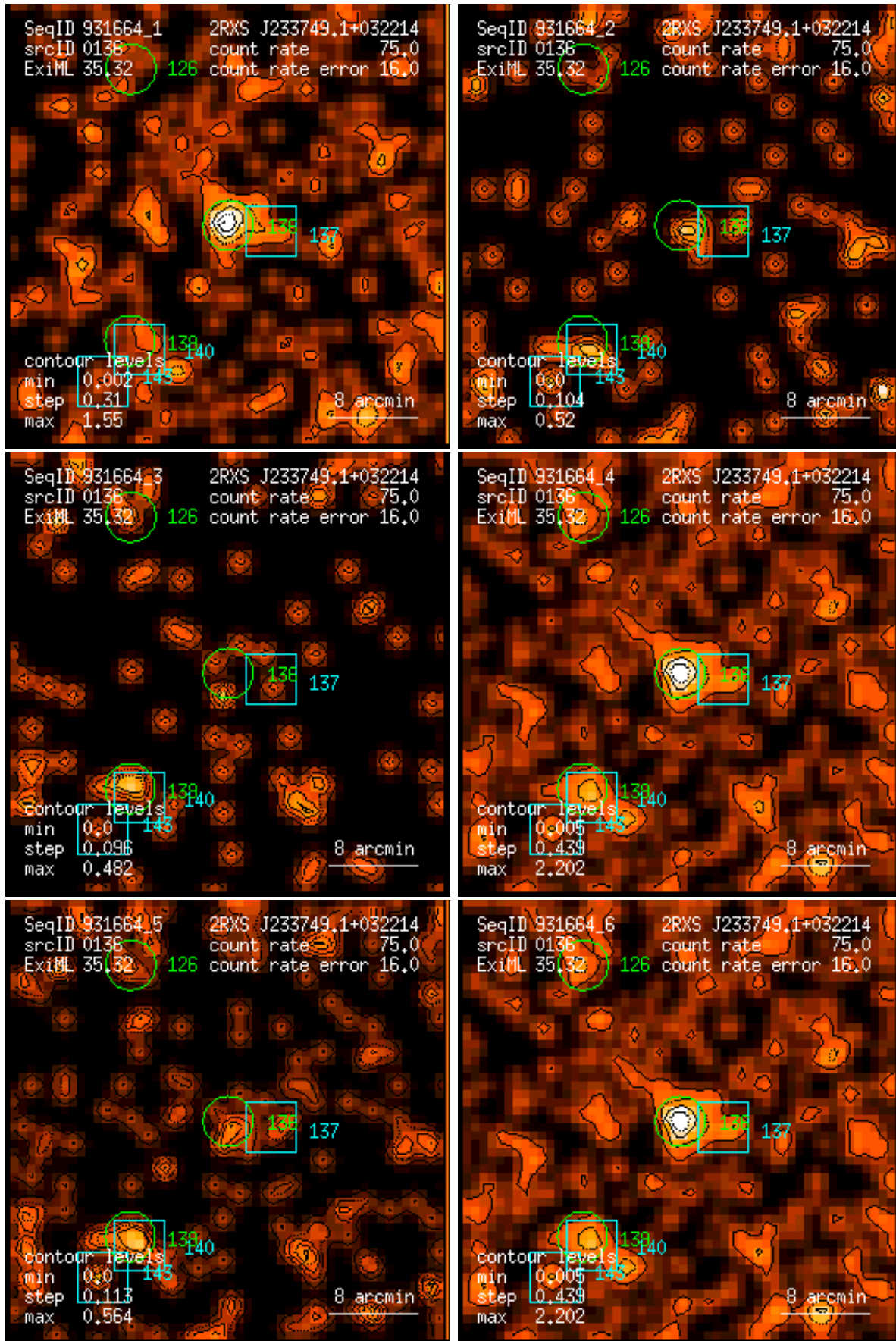
Figure 136: RASS 931664: detection 0136: band rate images, Gaussian filter: (1) PSPC channels 11 – 41, (2) 52 – 90, (3) 91 – 201, (4) 11 – 235, (5) 52 – 201, (6) 11 – 201. Broad band rates in counts/ks. Band rate contour levels in counts/ks/arcmin 2 .
