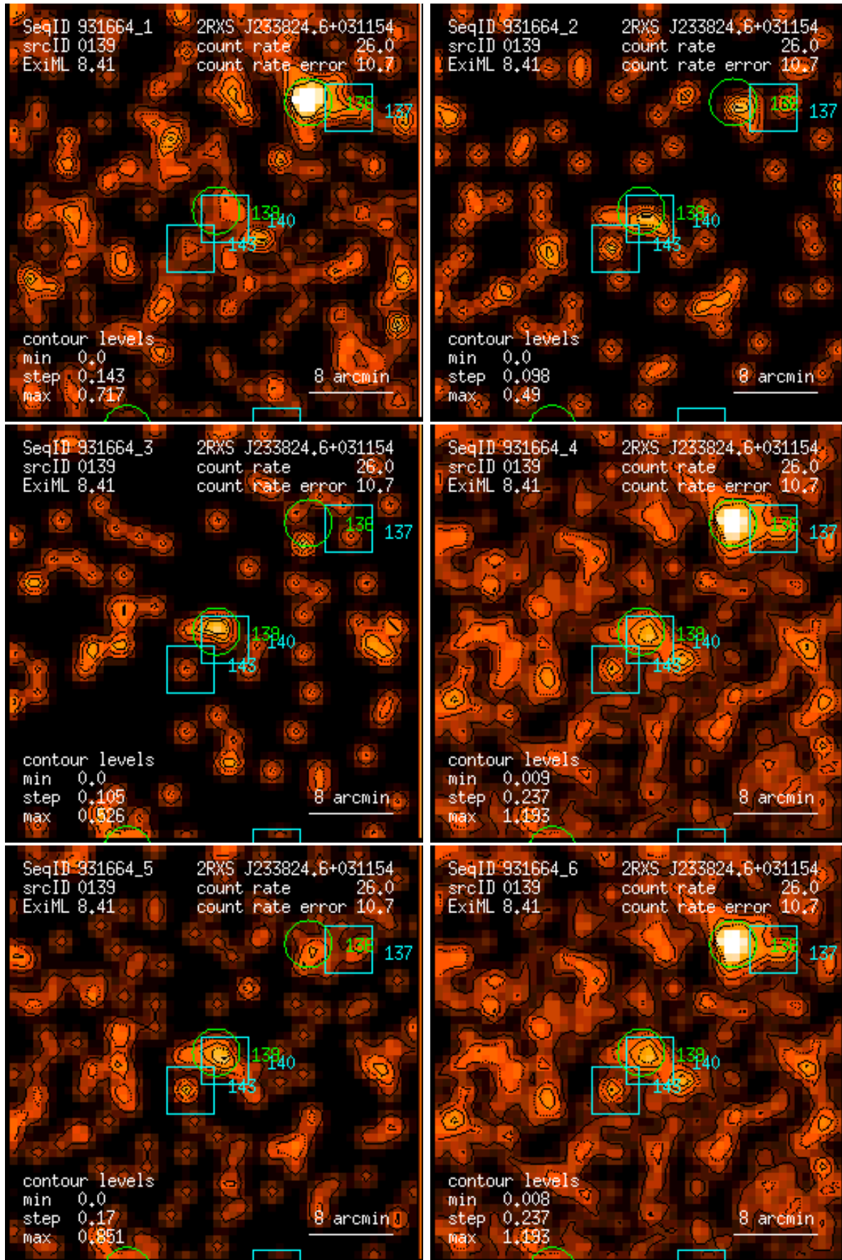
Figure 139: RASS 931664: detection 0139: band rate images, Gaussian filter: (1) PSPC channels 11 – 41, (2) 52 – 90, (3) 91 – 201, (4) 11 – 235, (5) 52 – 201, (6) 11 – 201. Broad band rates in counts/ks. Band rate contour levels in counts/ks/arcmin 2 .
