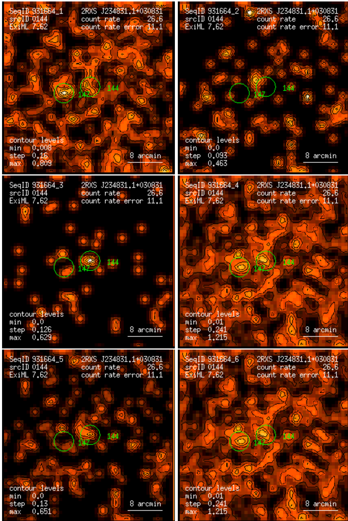
Figure 144: RASS 931664: detection 0144: band rate images, Gaussian filter: (1) PSPC channels 11 – 41, (2) 52 – 90, (3) 91 – 201, (4) 11 – 235, (5) 52 – 201, (6) 11 – 201. Broad band rates in counts/ks. Band rate contour levels in counts/ks/arcmin 2 .
