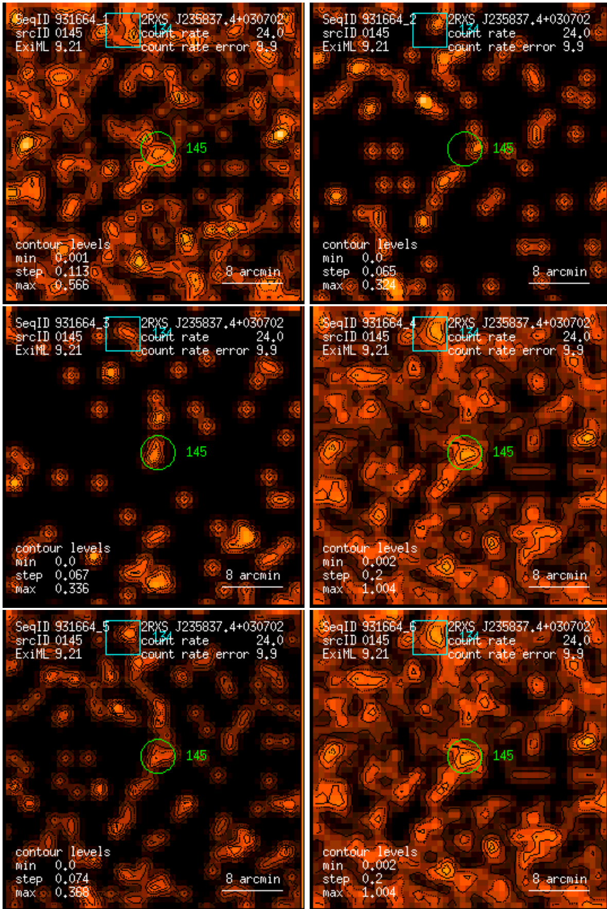
Figure 145: RASS 931664: detection 0145: band rate images, Gaussian filter: (1) PSPC channels 11 – 41, (2) 52 – 90, (3) 91 – 201, (4) 11 – 235, (5) 52 – 201, (6) 11 – 201. Broad band rates in counts/ks. Band rate contour levels in counts/ks/arcmin 2 .
