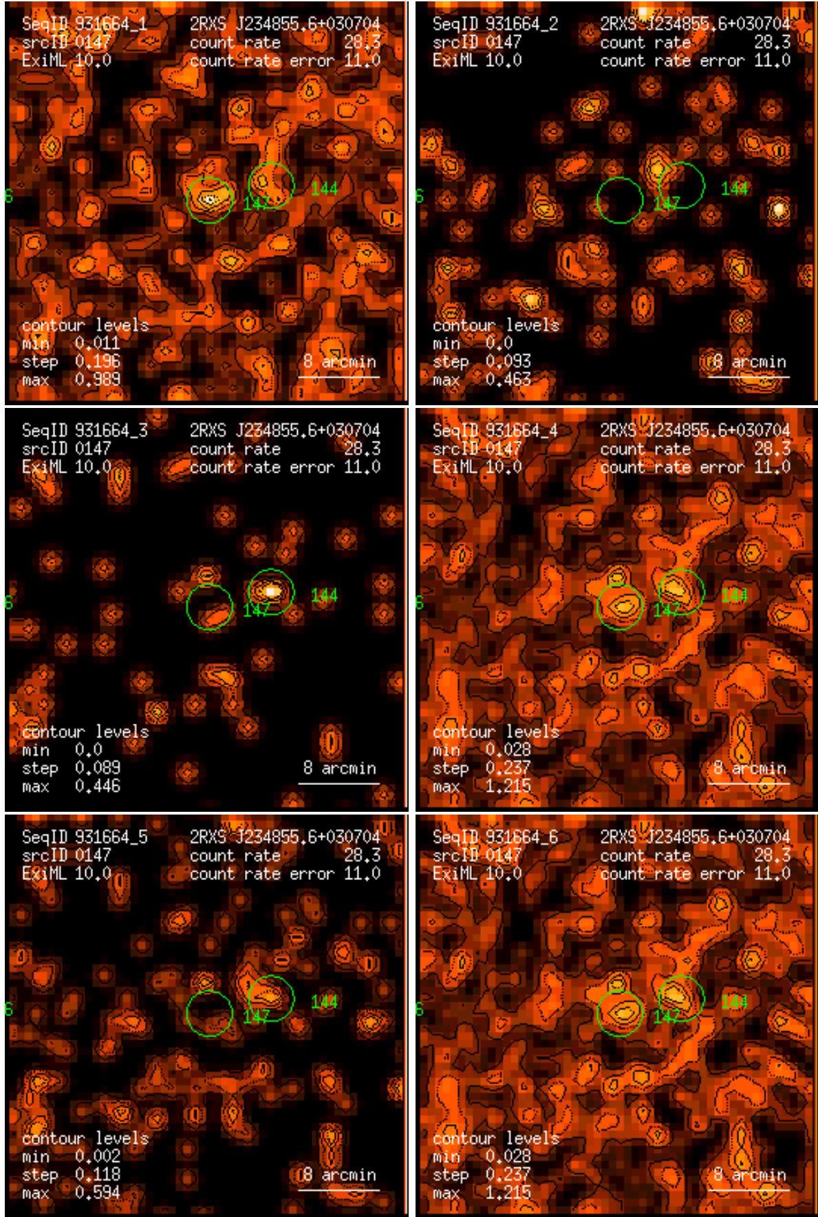
Figure 147: RASS 931664: detection 0147: band rate images, Gaussian filter: (1) PSPC channels 11 – 41, (2) 52 – 90, (3) 91 – 201, (4) 11 – 235, (5) 52 – 201, (6) 11 – 201. Broad band rates in counts/ks. Band rate contour levels in counts/ks/arcmin 2 .
