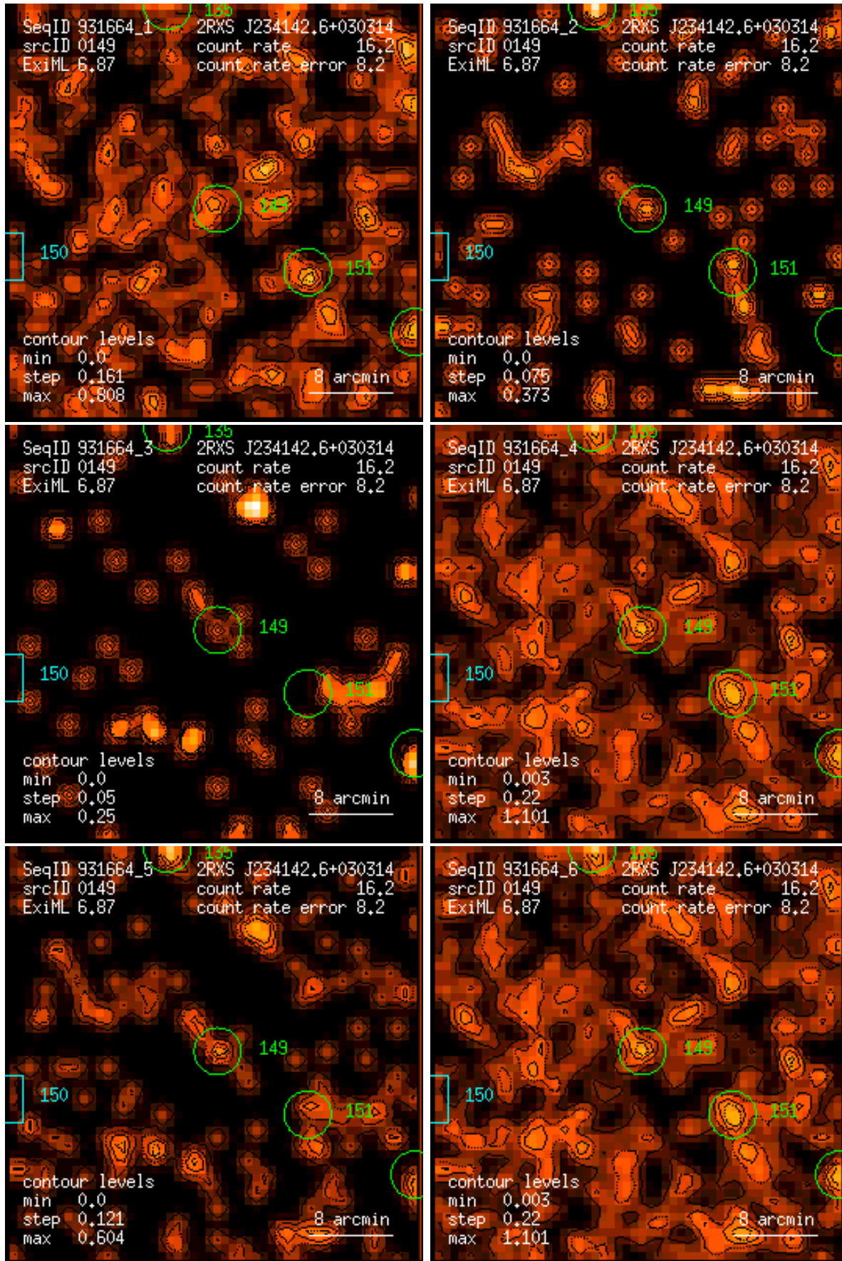
Figure 149: RASS 931664: detection 0149: band rate images, Gaussian filter: (1) PSPC channels 11 – 41, (2) 52 – 90, (3) 91 – 201, (4) 11 – 235, (5) 52 – 201, (6) 11 – 201. Broad band rates in counts/ks. Band rate contour levels in counts/ks/arcmin 2 .
