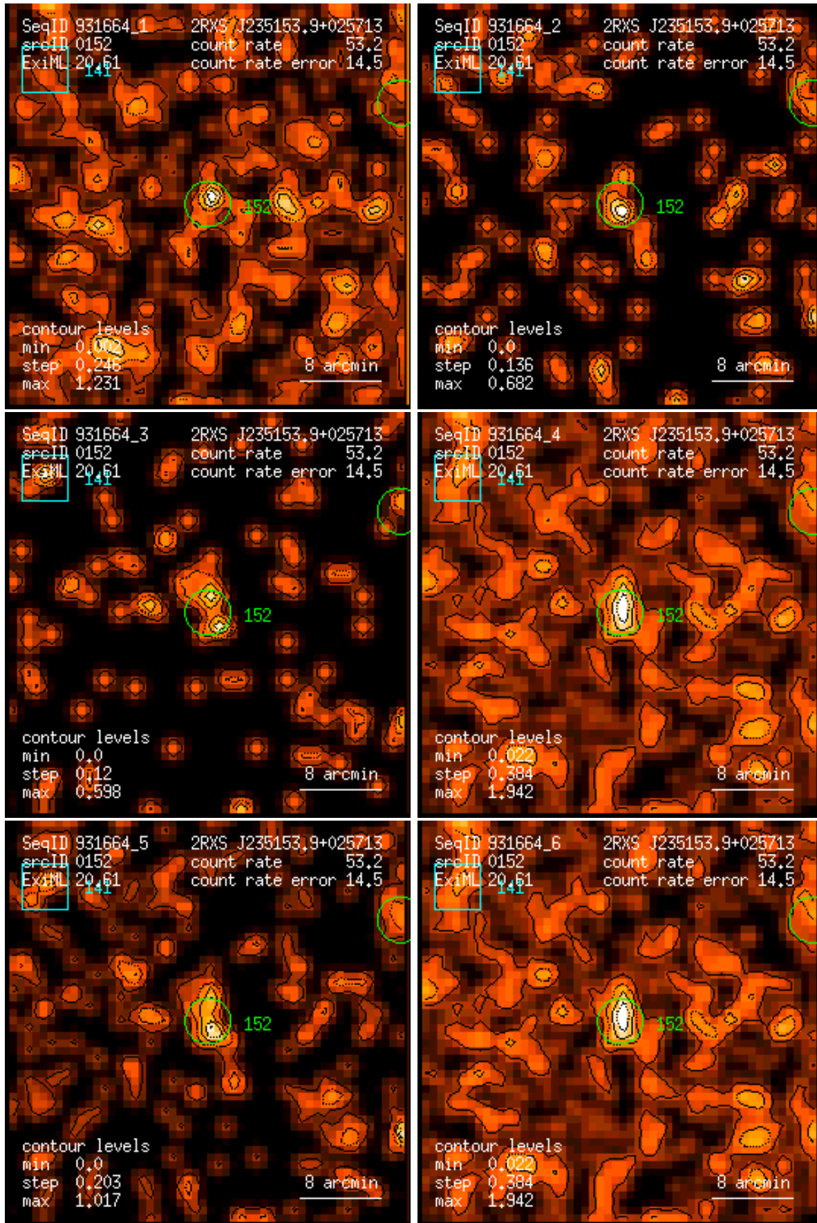
Figure 152: RASS 931664: detection 0152: band rate images, Gaussian filter: (1) PSPC channels 11 – 41, (2) 52 – 90, (3) 91 – 201, (4) 11 – 235, (5) 52 – 201, (6) 11 – 201. Broad band rates in counts/ks. Band rate contour levels in counts/ks/arcmin 2 .
