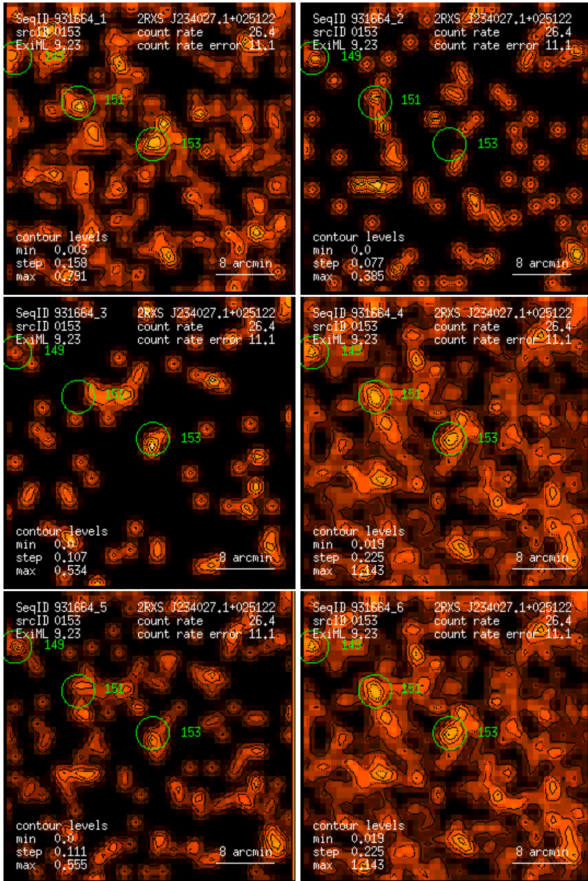
Figure 153: RASS 931664: detection 0153: band rate images, Gaussian filter: (1) PSPC channels 11 – 41, (2) 52 – 90, (3) 91 – 201, (4) 11 – 235, (5) 52 – 201, (6) 11 – 201. Broad band rates in counts/ks. Band rate contour levels in counts/ks/arcmin 2 .
