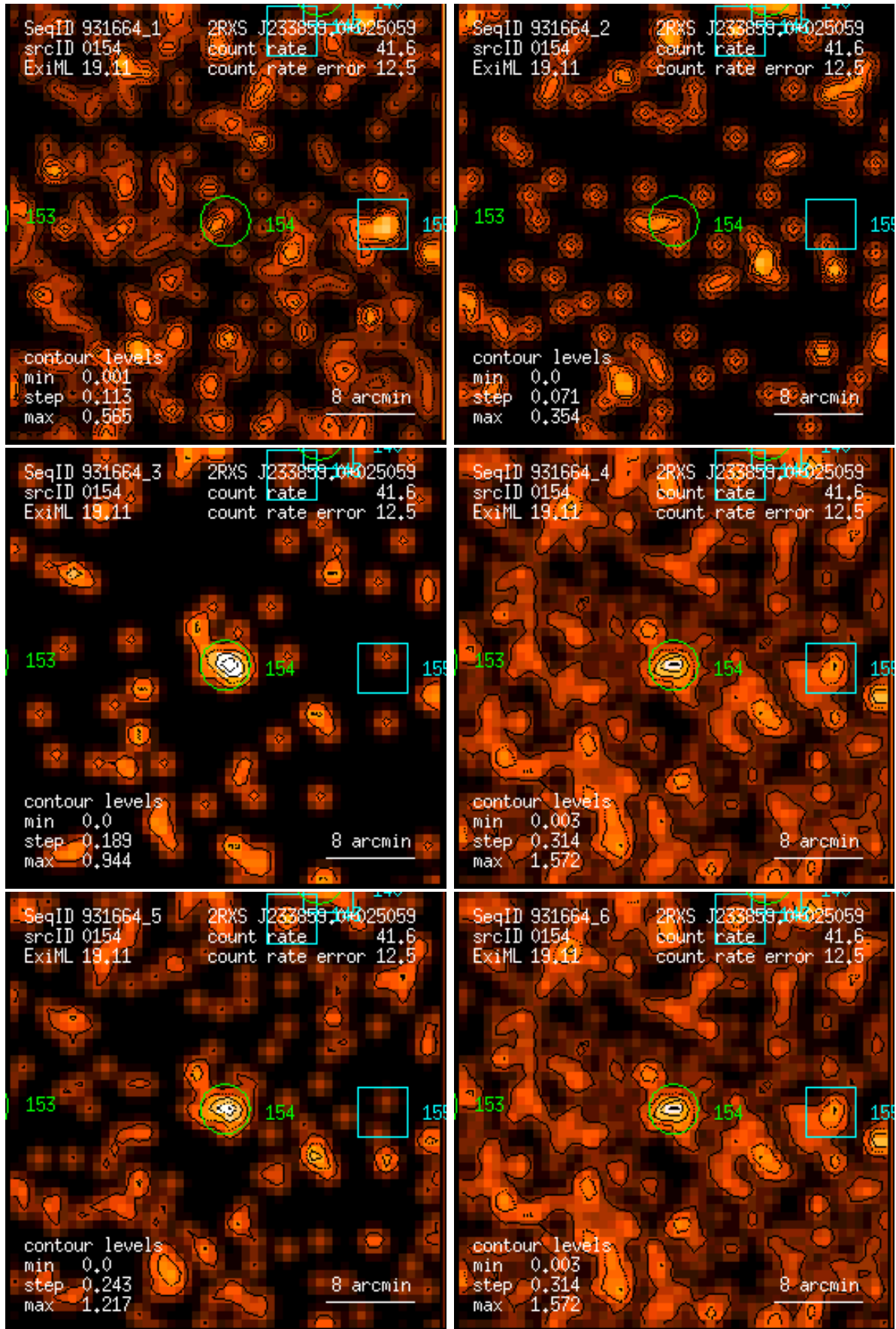
Figure 154: RASS 931664: detection 0154: band rate images, Gaussian filter: (1) PSPC channels 11 – 41, (2) 52 – 90, (3) 91 – 201, (4) 11 – 235, (5) 52 – 201, (6) 11 – 201. Broad band rates in counts/ks. Band rate contour levels in counts/ks/arcmin 2 .
