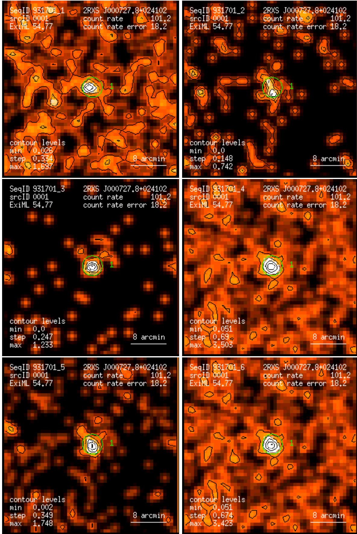
Figure 1: RASS 931701: detection 0001: band rate images, Gaussian filter: (1) PSPC channels 11 – 41, (2) 52 – 90, (3) 91 – 201, (4) 11 – 235, (5) 52 – 201, (6) 11 – 201. Broad band rates in counts/ks. Band rate contour levels in counts/ks/arcmin 2 .
