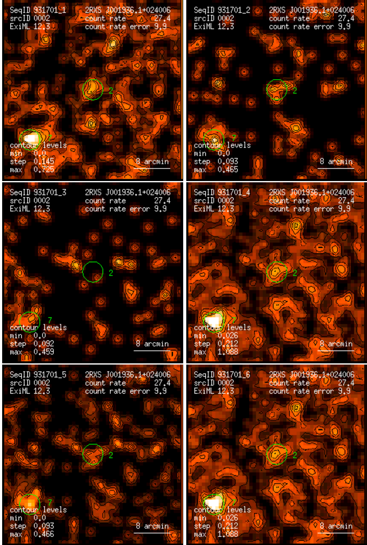
Figure 2: RASS 931701: detection 0002: band rate images, Gaussian filter: (1) PSPC channels 11 – 41, (2) 52 – 90, (3) 91 – 201, (4) 11 – 235, (5) 52 – 201, (6) 11 – 201. Broad band rates in counts/ks. Band rate contour levels in counts/ks/arcmin 2 .
