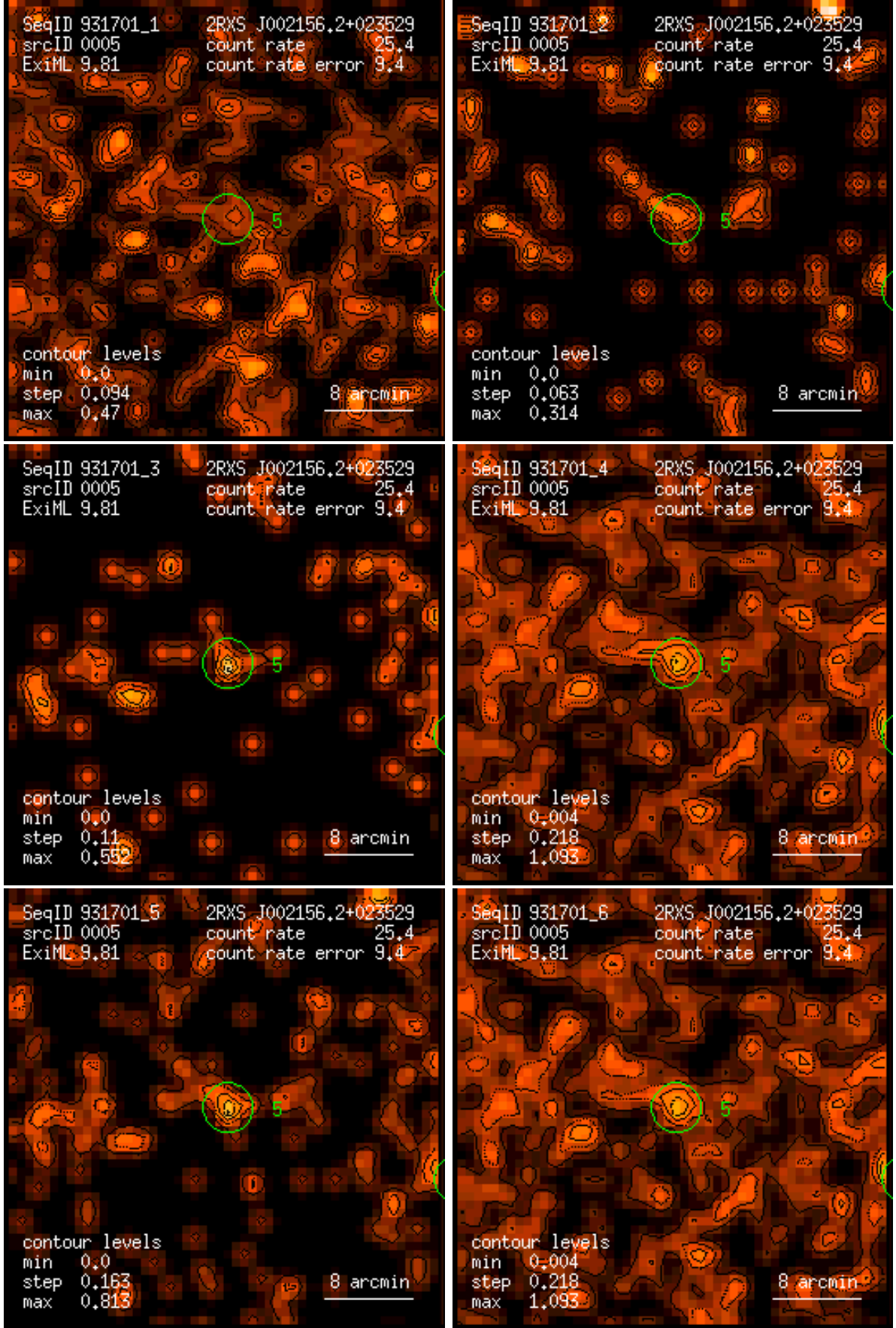
Figure 5: RASS 931701: detection 0005: band rate images, Gaussian filter: (1) PSPC channels 11 – 41, (2) 52 – 90, (3) 91 – 201, (4) 11 – 235, (5) 52 – 201, (6) 11 – 201. Broad band rates in counts/ks. Band rate contour levels in counts/ks/arcmin 2 .
