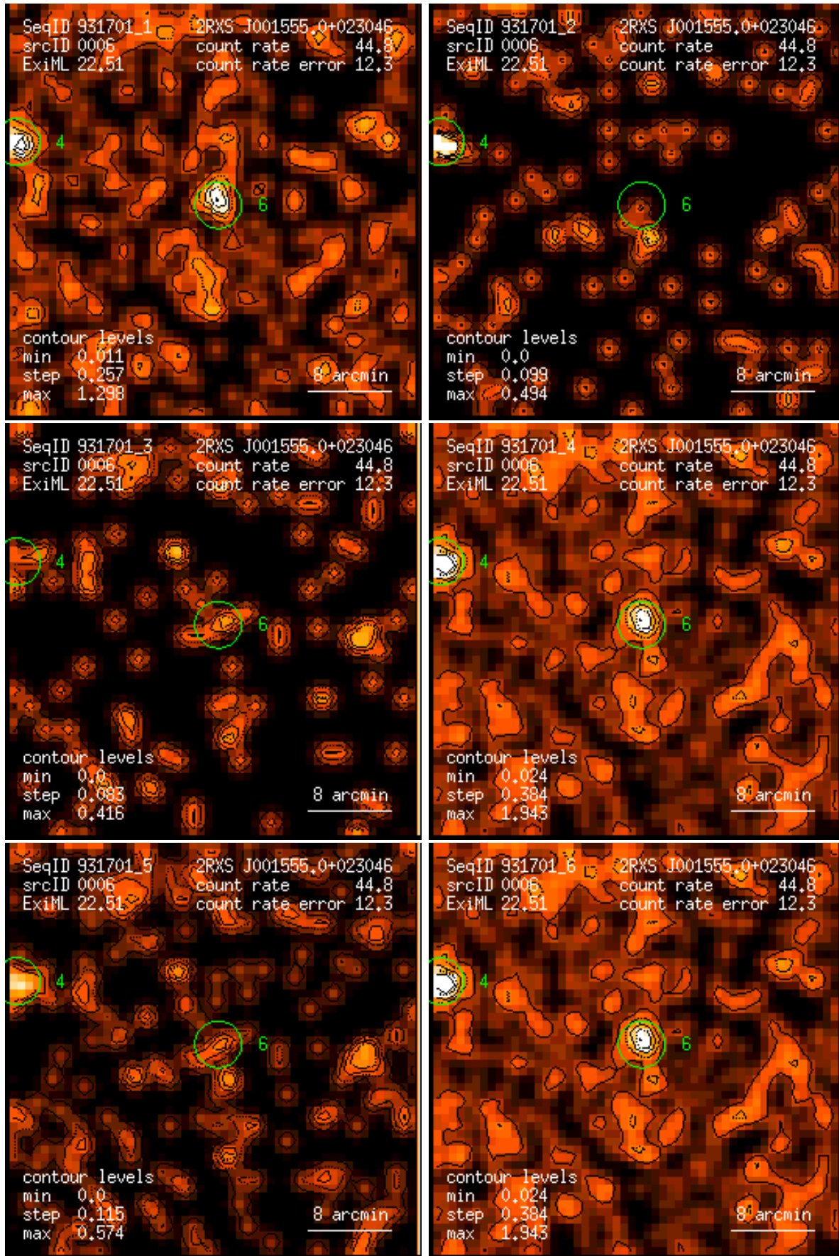
Figure 6: RASS 931701: detection 0006: band rate images, Gaussian filter: (1) PSPC channels 11 – 41, (2) 52 – 90, (3) 91 – 201, (4) 11 – 235, (5) 52 – 201, (6) 11 – 201. Broad band rates in counts/ks. Band rate contour levels in counts/ks/arcmin 2 .
