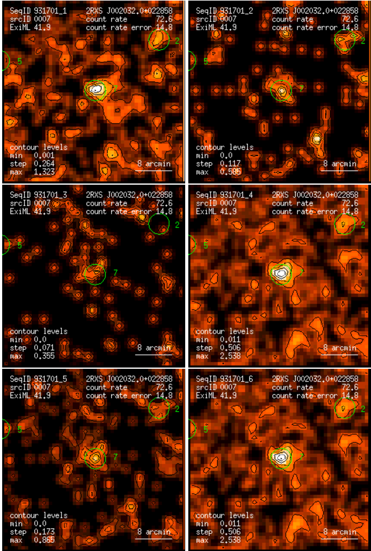
Figure 7: RASS 931701: detection 0007: band rate images, Gaussian filter: (1) PSPC channels 11 – 41, (2) 52 – 90, (3) 91 – 201, (4) 11 – 235, (5) 52 – 201, (6) 11 – 201. Broad band rates in counts/ks. Band rate contour levels in counts/ks/arcmin 2 .
