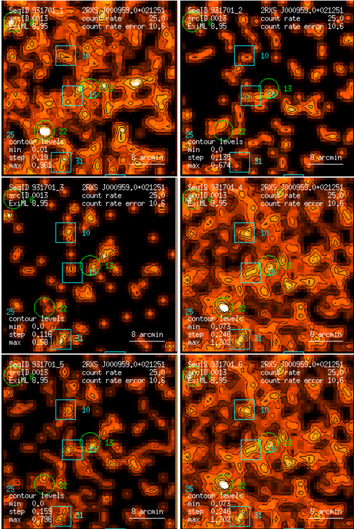
Figure 13: RASS 931701: detection 0013: band rate images, Gaussian filter: (1) PSPC channels 11 – 41, (2) 52 – 90, (3) 91 – 201, (4) 11 – 235, (5) 52 – 201, (6) 11 – 201. Broad band rates in counts/ks. Band rate contour levels in counts/ks/arcmin 2 .
