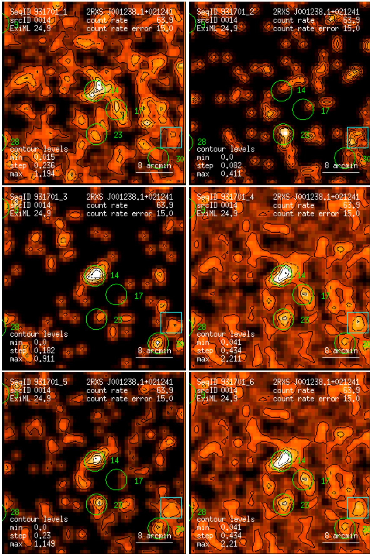
Figure 14: RASS 931701: detection 0014: band rate images, Gaussian filter: (1) PSPC channels 11 – 41, (2) 52 – 90, (3) 91 – 201, (4) 11 – 235, (5) 52 – 201, (6) 11 – 201. Broad band rates in counts/ks. Band rate contour levels in counts/ks/arcmin 2 .
