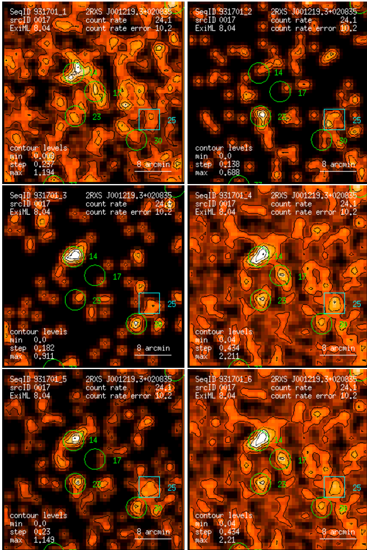
Figure 17: RASS 931701: detection 0017: band rate images, Gaussian filter: (1) PSPC channels 11 – 41, (2) 52 – 90, (3) 91 – 201, (4) 11 – 235, (5) 52 – 201, (6) 11 – 201. Broad band rates in counts/ks. Band rate contour levels in counts/ks/arcmin 2 .
