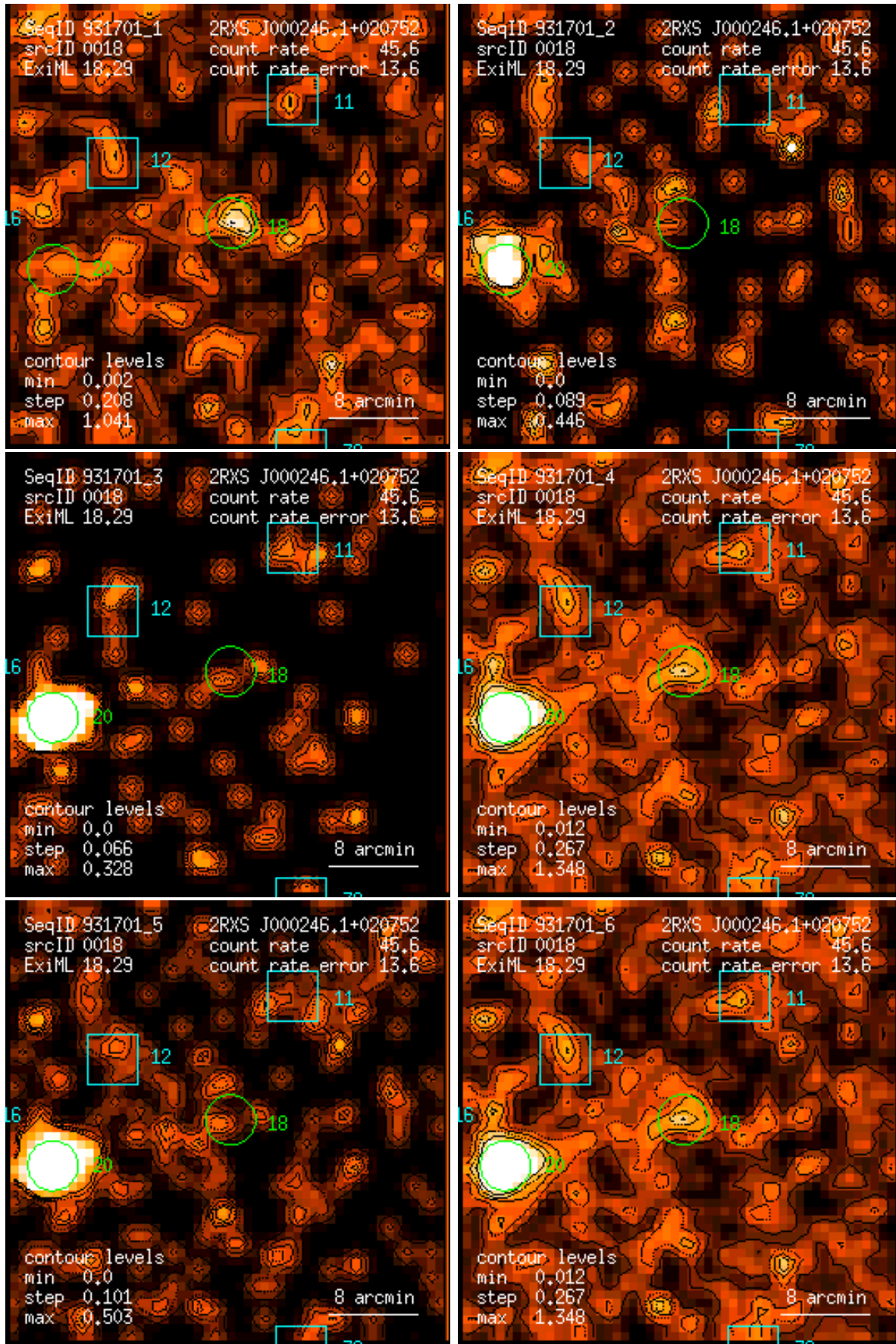
Figure 18: RASS 931701: detection 0018: band rate images, Gaussian filter: (1) PSPC channels 11 – 41, (2) 52 – 90, (3) 91 – 201, (4) 11 – 235, (5) 52 – 201, (6) 11 – 201. Broad band rates in counts/ks. Band rate contour levels in counts/ks/arcmin 2 .
