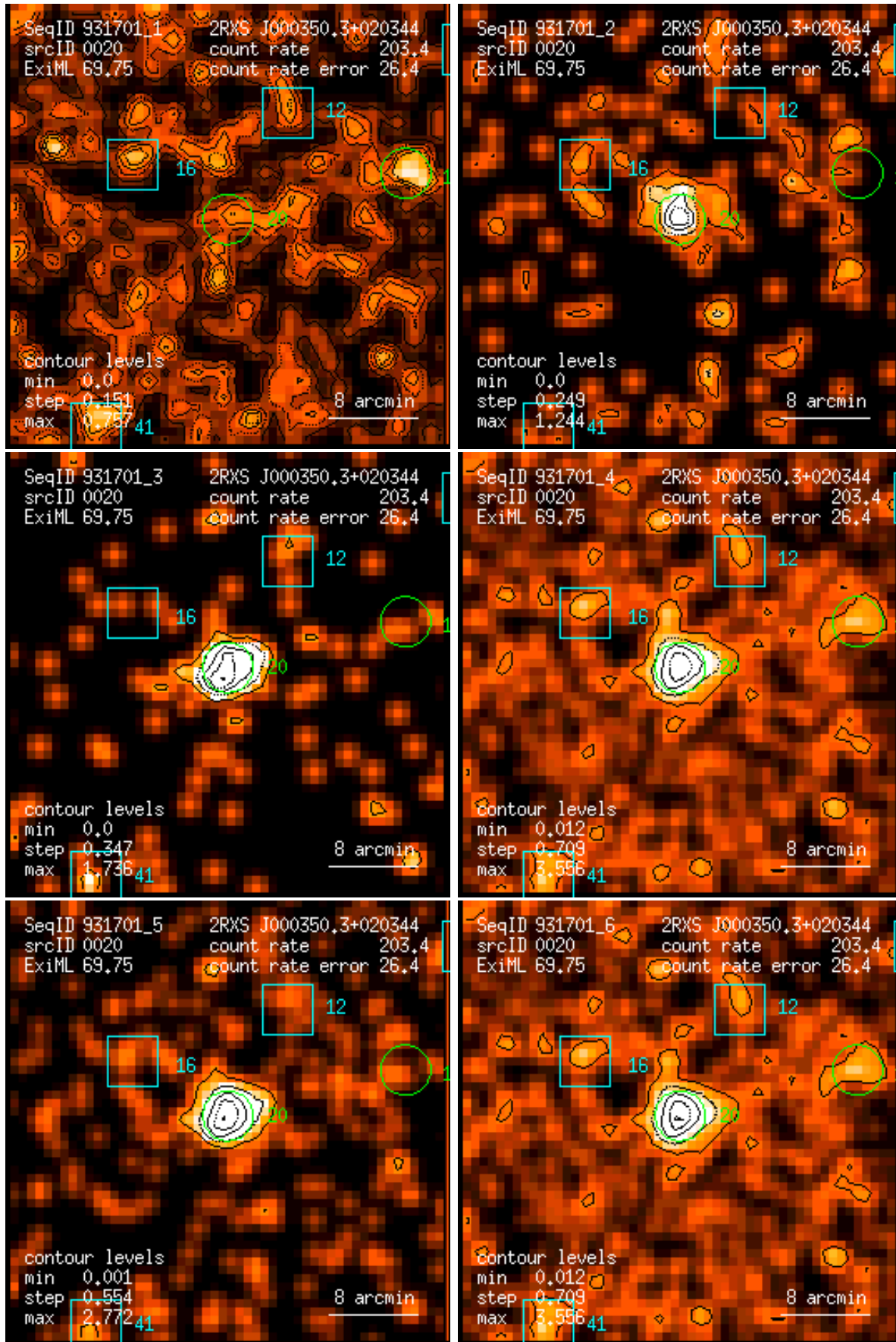
Figure 20: RASS 931701: detection 0020: band rate images, Gaussian filter: (1) PSPC channels 11 – 41, (2) 52 – 90, (3) 91 – 201, (4) 11 – 235, (5) 52 – 201, (6) 11 – 201. Broad band rates in counts/ks. Band rate contour levels in counts/ks/arcmin 2 .
