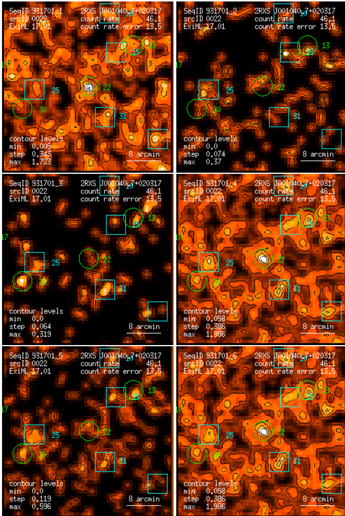
Figure 22: RASS 931701: detection 0022: band rate images, Gaussian filter: (1) PSPC channels 11 – 41, (2) 52 – 90, (3) 91 – 201, (4) 11 – 235, (5) 52 – 201, (6) 11 – 201. Broad band rates in counts/ks. Band rate contour levels in counts/ks/arcmin 2 .
