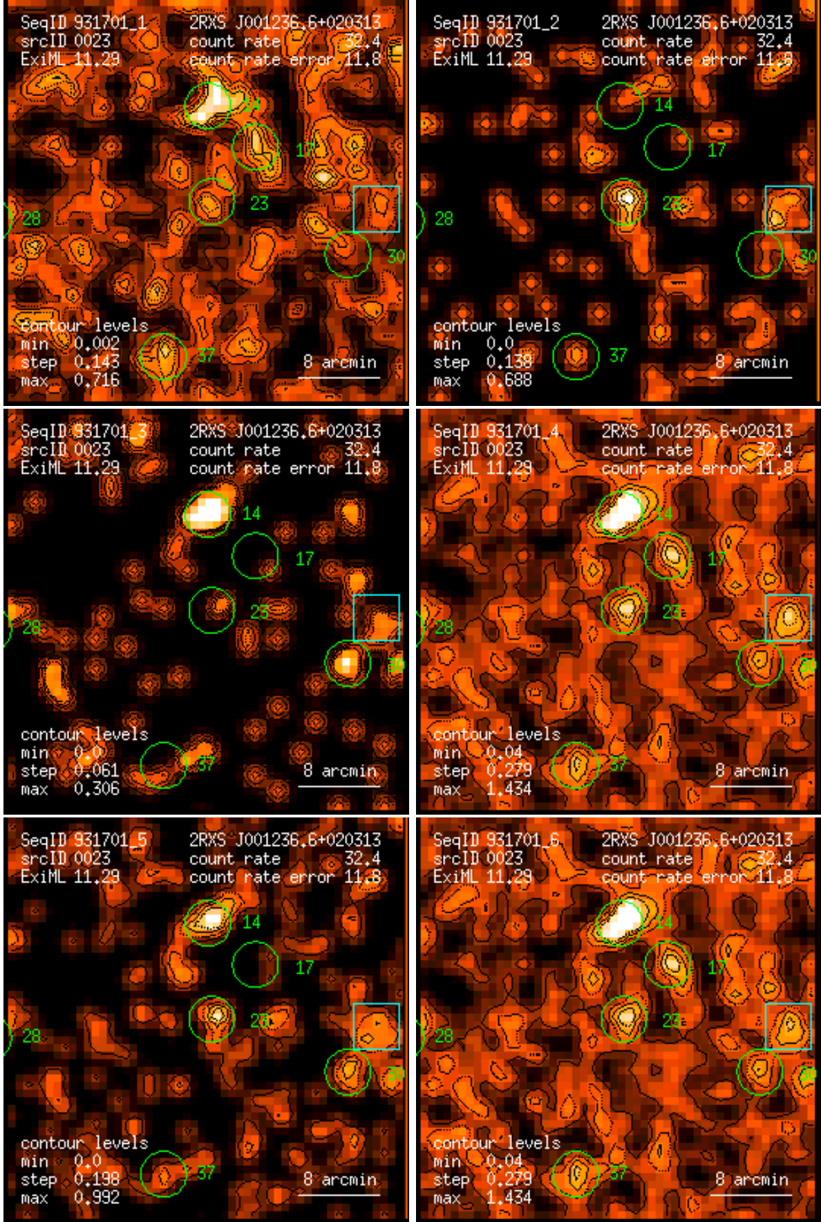
Figure 23: RASS 931701: detection 0023: band rate images, Gaussian filter: (1) PSPC channels 11 – 41, (2) 52 – 90, (3) 91 – 201, (4) 11 – 235, (5) 52 – 201, (6) 11 – 201. Broad band rates in counts/ks. Band rate contour levels in counts/ks/arcmin 2 .
