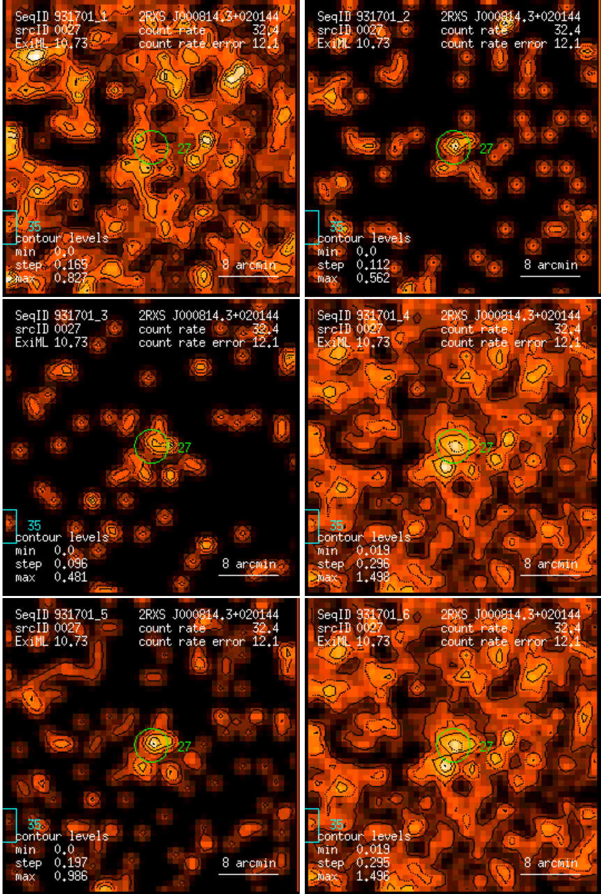
Figure 27: RASS 931701: detection 0027: band rate images, Gaussian filter: (1) PSPC channels 11 – 41, (2) 52 – 90, (3) 91 – 201, (4) 11 – 235, (5) 52 – 201, (6) 11 – 201. Broad band rates in counts/ks. Band rate contour levels in counts/ks/arcmin 2 .
