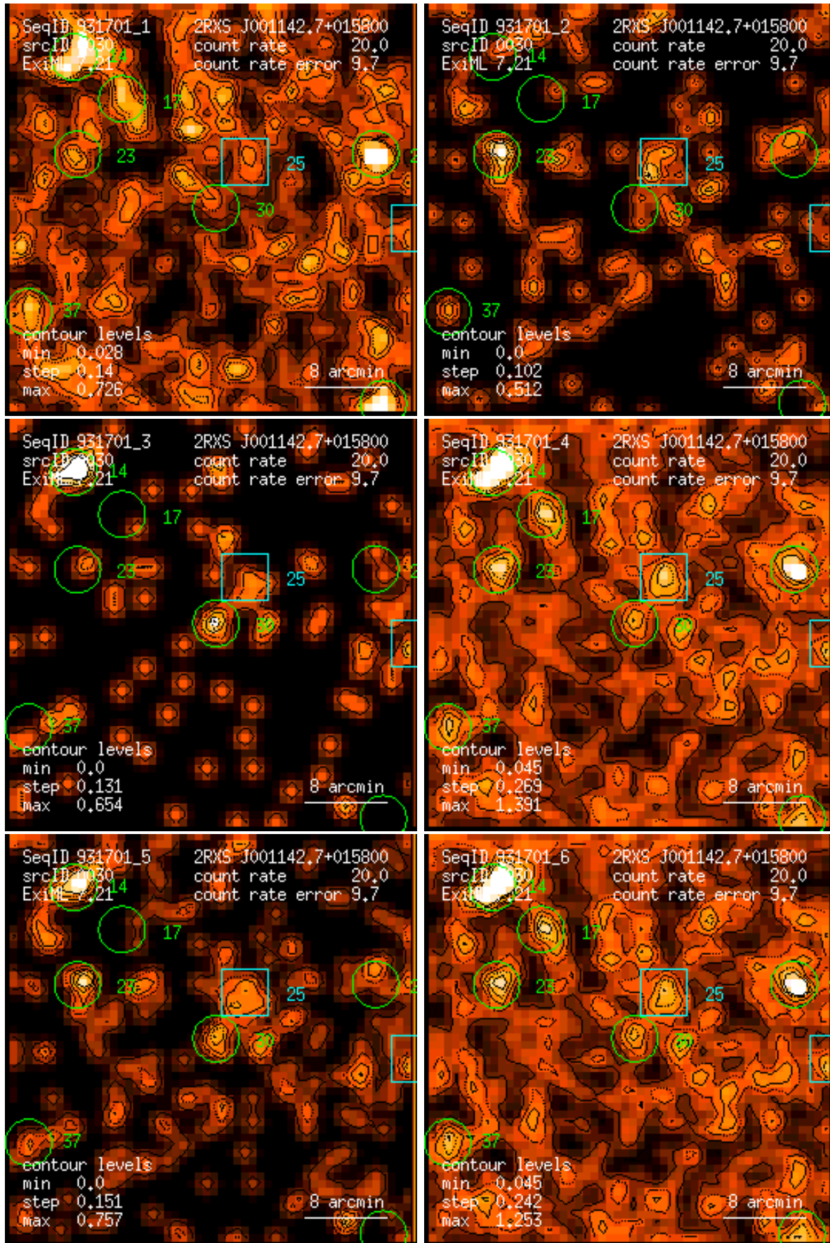
Figure 30: RASS 931701: detection 0030: band rate images, Gaussian filter: (1) PSPC channels 11 – 41, (2) 52 – 90, (3) 91 – 201, (4) 11 – 235, (5) 52 – 201, (6) 11 – 201. Broad band rates in counts/ks. Band rate contour levels in counts/ks/arcmin 2 .
