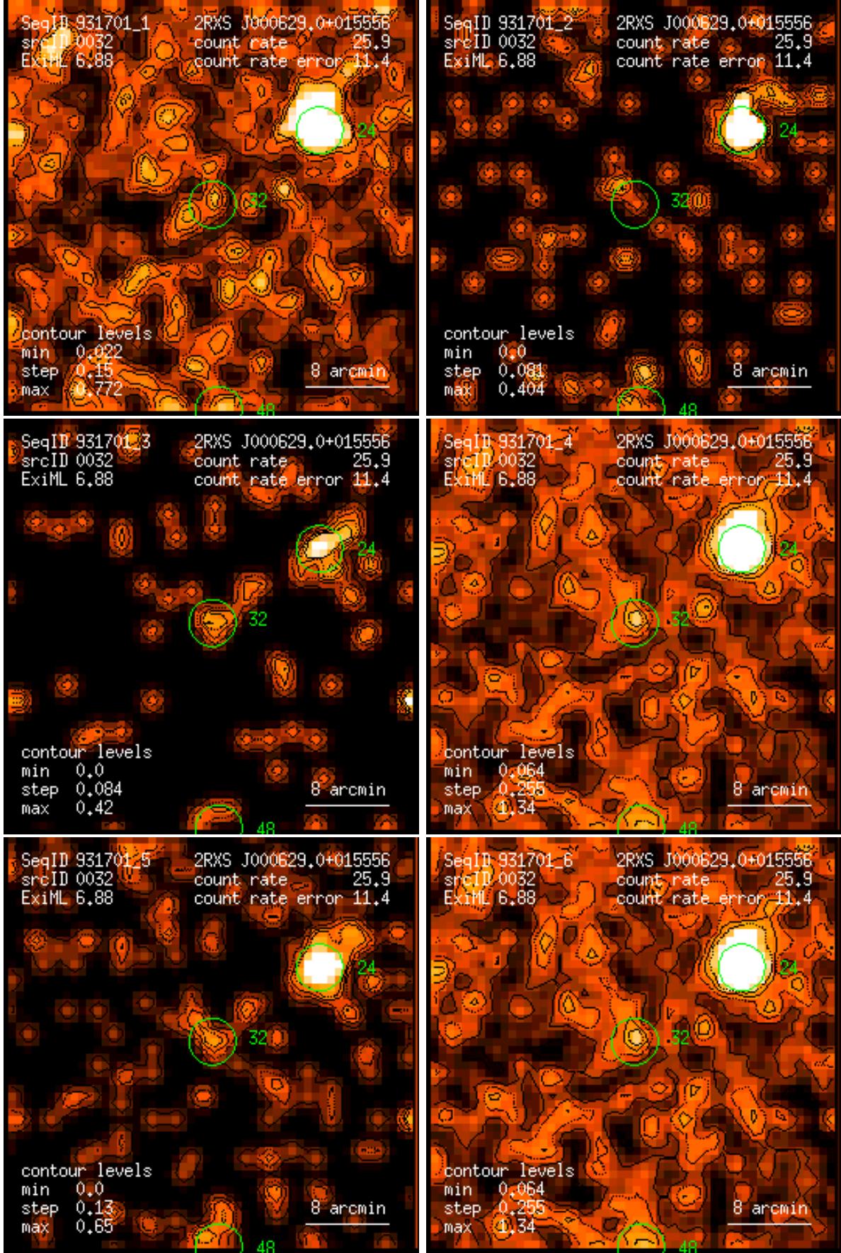
Figure 32: RASS 931701: detection 0032: band rate images, Gaussian filter: (1) PSPC channels 11 – 41, (2) 52 – 90, (3) 91 – 201, (4) 11 – 235, (5) 52 – 201, (6) 11 – 201. Broad band rates in counts/ks. Band rate contour levels in counts/ks/arcmin 2 .
